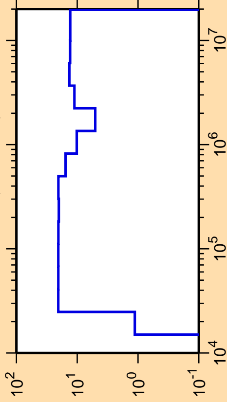
\Delta\sigma/\sigma vs. E for ^{60}\text{Mn}(n,\text{nonel.})
