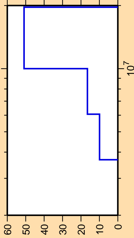
\Delta\sigma/\sigma vs. E for ^{60}\text{Mn}(n,n\text{cont.})
