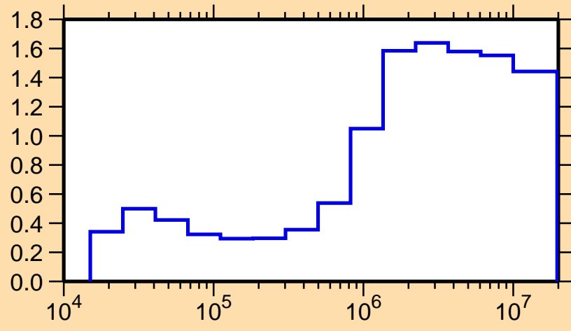
\sigma vs. E for ^{60}\text{Mn}(n,\text{nonel.})
