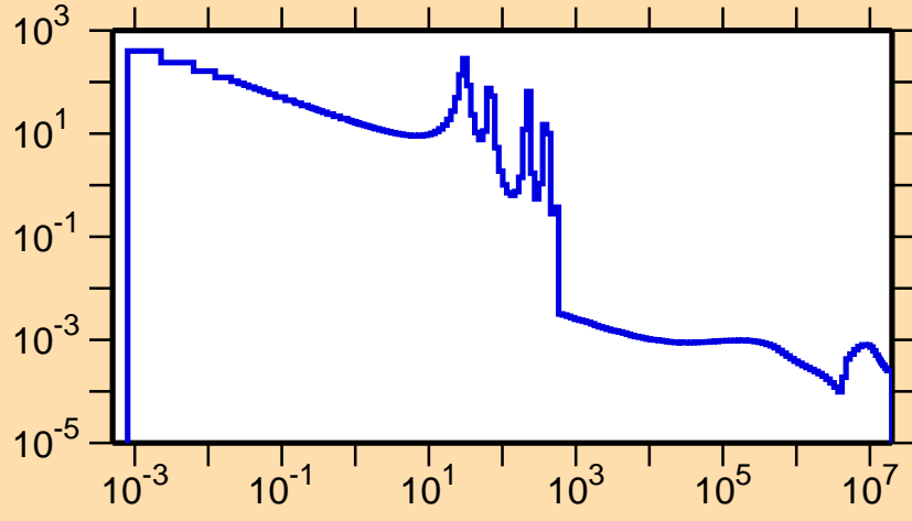
\sigma vs. E for ^{84}\text{Mo}(n,\gamma)
