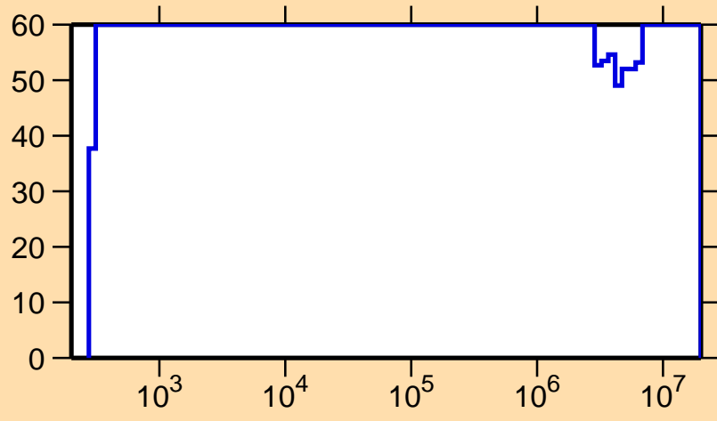
\Delta\sigma/\sigma vs. E for ^{84}\text{Mo}(n,\gamma)
