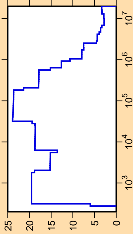
\Delta\sigma/\sigma vs. E for ^{84}\text{Mo}(n,\text{nonel.})
