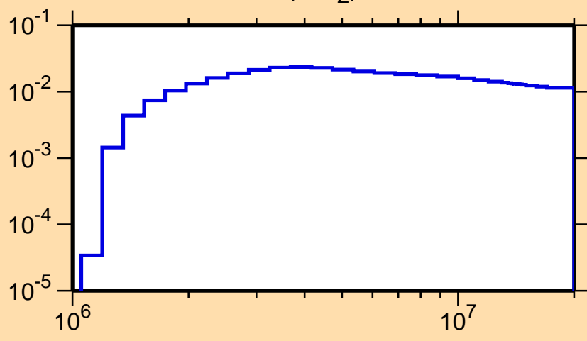
\sigma vs. E for ^{84}\text{Mo}(n,n_2)
