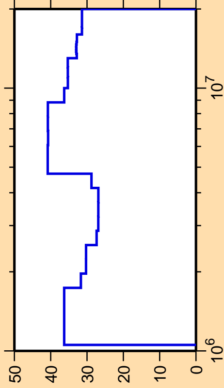
\Delta\sigma/\sigma vs. E for ^{84}\text{Mo}(n,n_2)
