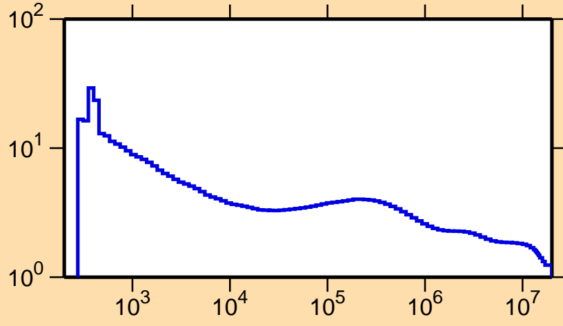
\sigma vs. E for ^{84}\text{Mo}(n,\text{nonel.})
