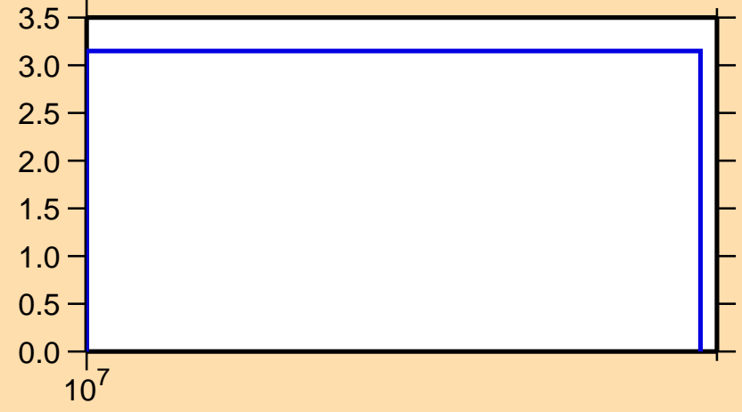
\Delta\sigma/\sigma vs. E for ^{84}\text{Mo}(n,\text{nonel.})
