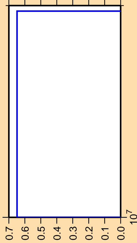
\Delta\sigma/\sigma vs. E for ^{84}\text{Mo}(n,nd)
