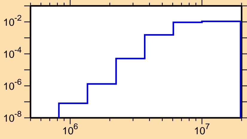
\sigma vs. E for ^{84}\text{Mo}(n,n\text{cont.})
