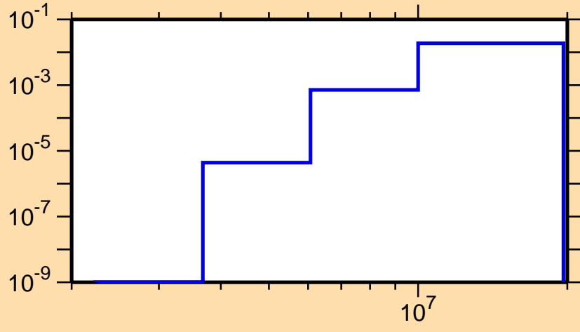
\sigma vs. E for ^{84}\text{Mo}(n,d)
