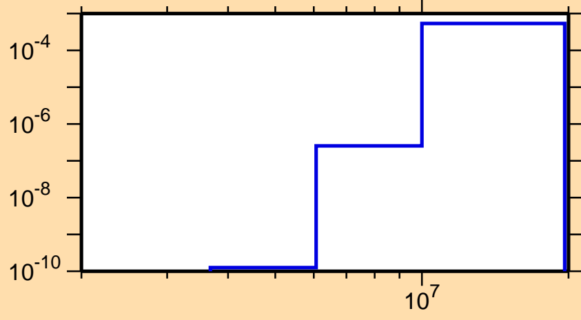
\sigma vs. E for ^{84}\text{Mo}(n,n\alpha)
