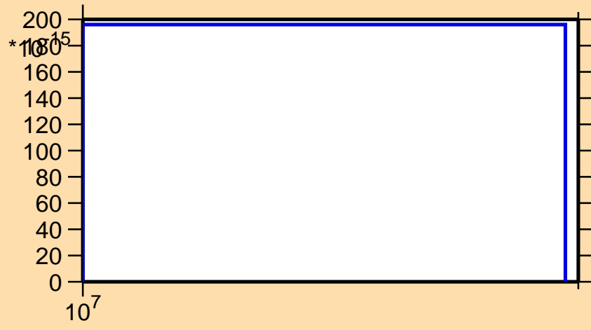
\sigma vs. E for ^{84}\text{Mo}(n,nd)
