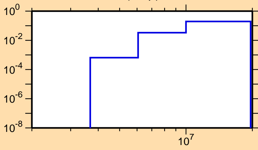
\sigma vs. E for ^{84}\text{Mo}(n,np)
