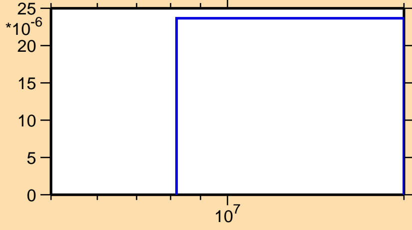
\sigma vs. E for ^{84}\text{Mo}(n,t)
