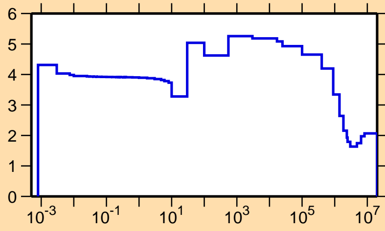
\sigma vs. E for ^{84}\text{Mo}(n,\text{el.})
