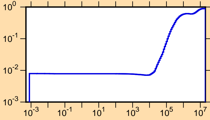
\mu vs. E for ^{85}\text{Mo}(\text{mt251})
