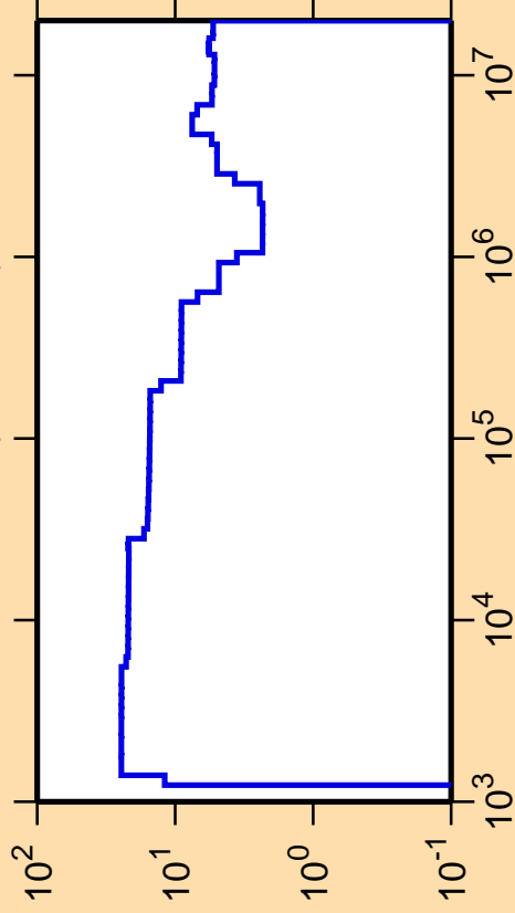
\Delta\sigma/\sigma vs. E for ^{85}\text{Mo}(n,\text{nonel.})
