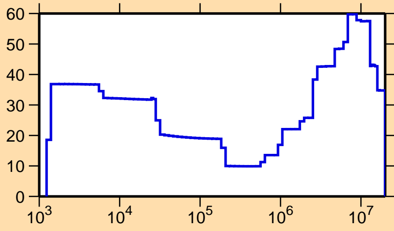
\Delta\sigma/\sigma vs. E for ^{85}\text{Mo}(n,p)
