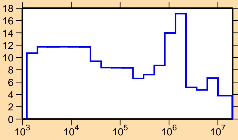
\Delta\sigma/\sigma vs. E for ^{85}\text{Mo}(n,el.)
