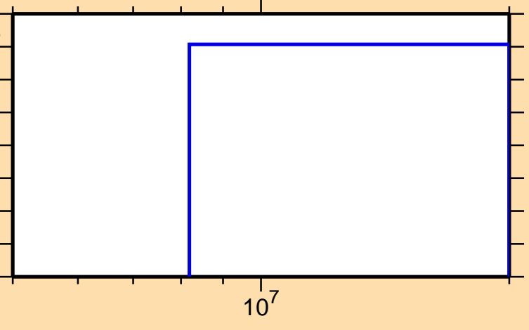
\sigma vs. E for ^{85}\text{Mo}(n,2n)
