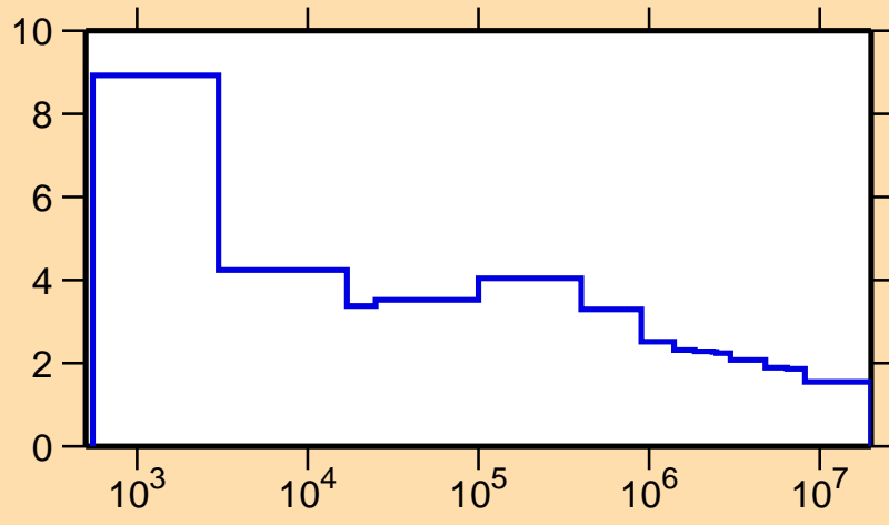
\sigma vs. E for ^{85}\text{Mo}(n,\text{nonel.})
