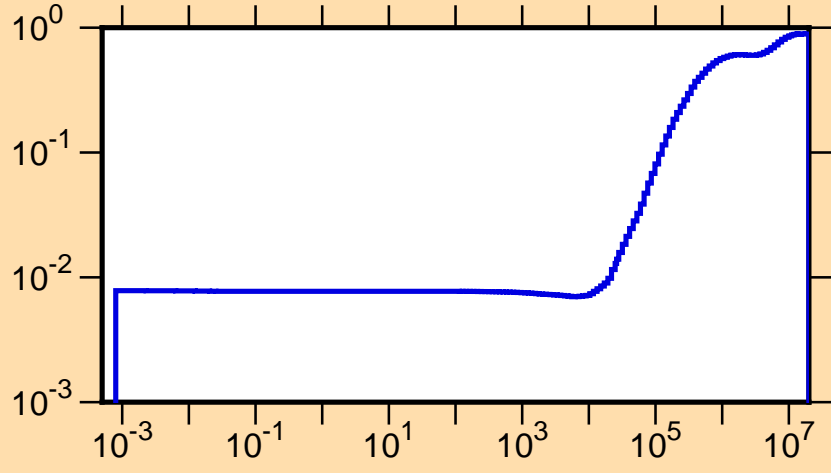
\mu vs. E for ^{86}\text{Mo}(\text{mt251})
