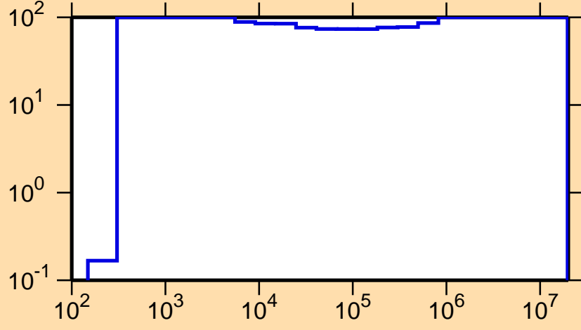
\Delta\sigma/\sigma vs. E for ^{86}\text{Mo}(n,\gamma)
