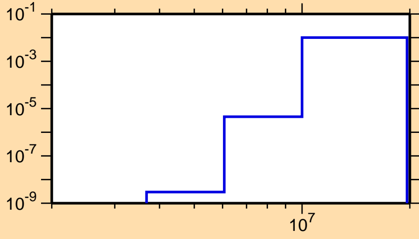
\sigma vs. E for ^{86}\text{Mo}(n,d)
