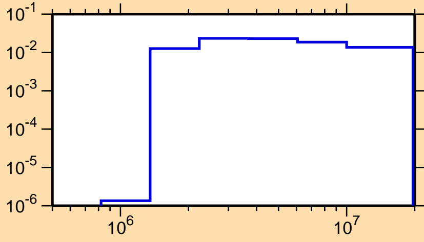
\sigma vs. E for ^{86}\text{Mo}(n,n_2)
