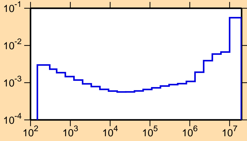
\sigma vs. E for ^{86}\text{Mo}(n,\alpha)
