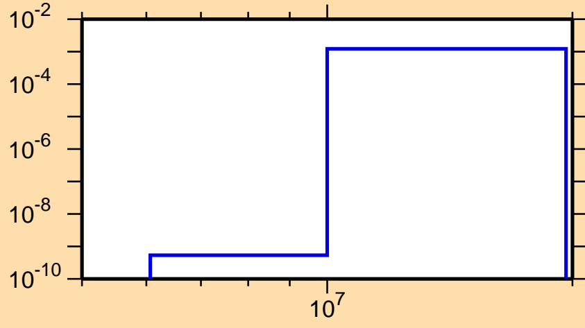
\sigma vs. E for ^{86}\text{Mo}(n,\text{pd})
