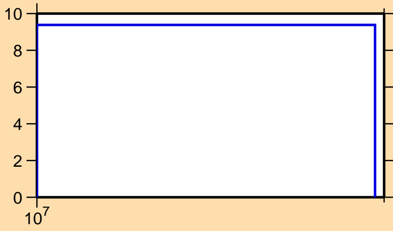
\Delta\sigma/\sigma vs. E for ^{86}\text{Mo}(n,\text{tot.})
