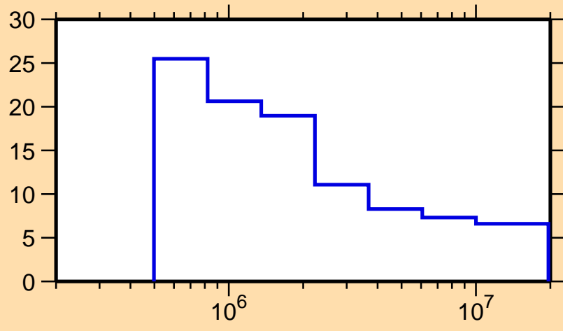
\Delta\sigma/\sigma vs. E for ^{86}\text{Mo}(n,\text{nonel.})
