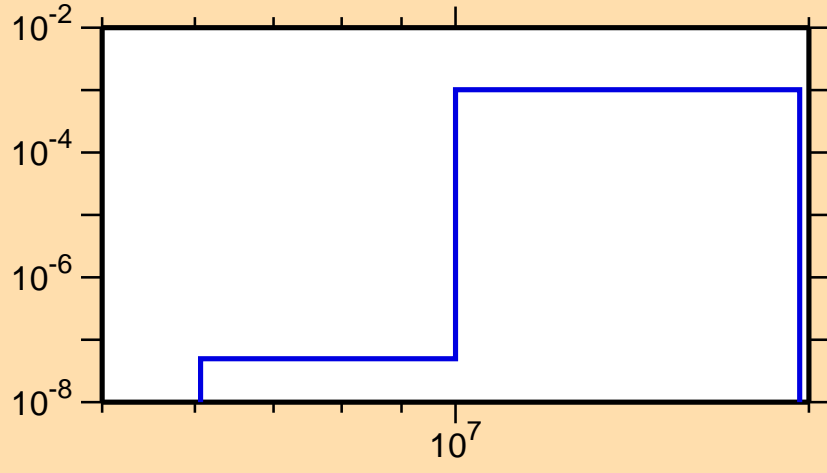
\sigma vs. E for ^{86}\text{Mo}(n,n\alpha)
