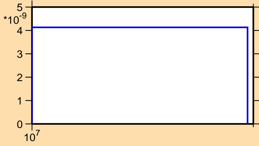
\sigma vs. E for ^{86}\text{Mo}(n,\text{pt})
