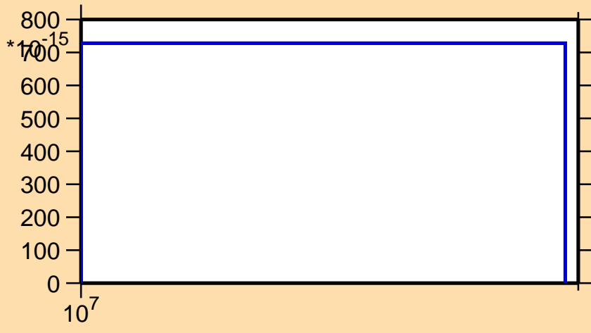
\sigma vs. E for ^{86}\text{Mo}(n,\text{nd})
