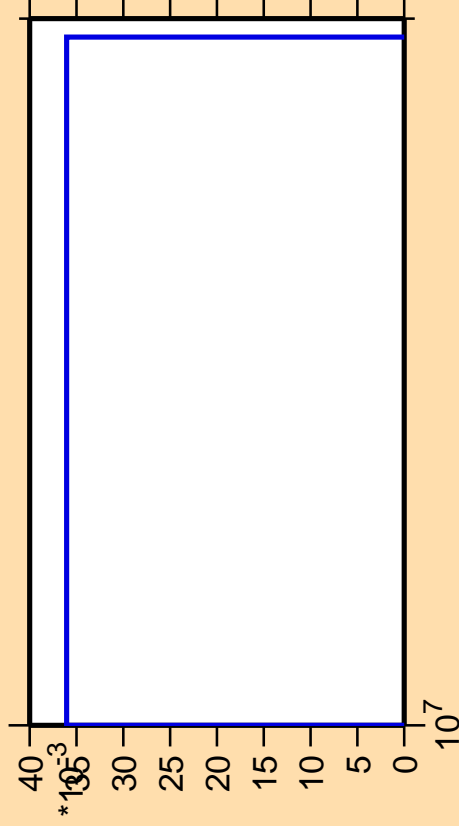
\Delta\sigma/\sigma vs. E for ^{86}\text{Mo}(n,2np)
