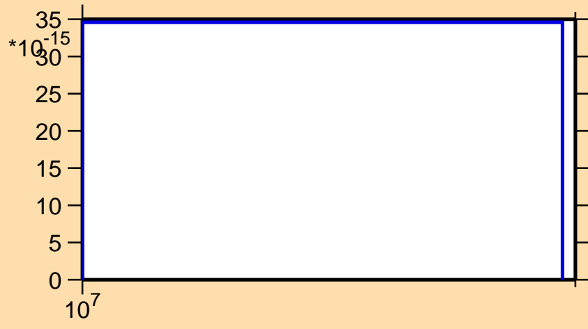
\sigma vs. E for ^{86}\text{Mo}(n,2np)
