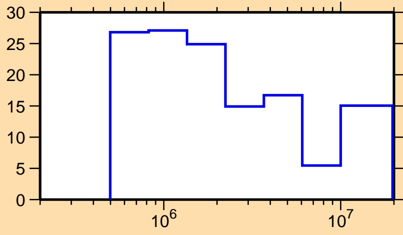
\Delta\sigma/\sigma vs. E for ^{86}\text{Mo}(n,\text{el.})
