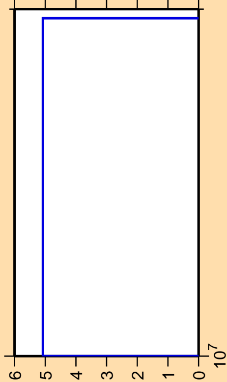
\Delta\sigma/\sigma vs. E for ^{86}\text{Mo}(n,\text{nd})
