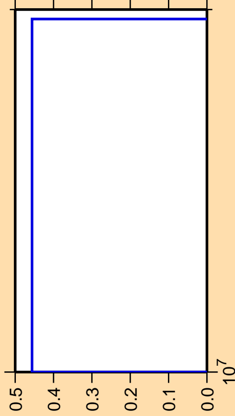
\Delta\sigma/\sigma vs. E for ^{86}\text{Mo} (mt 34)
