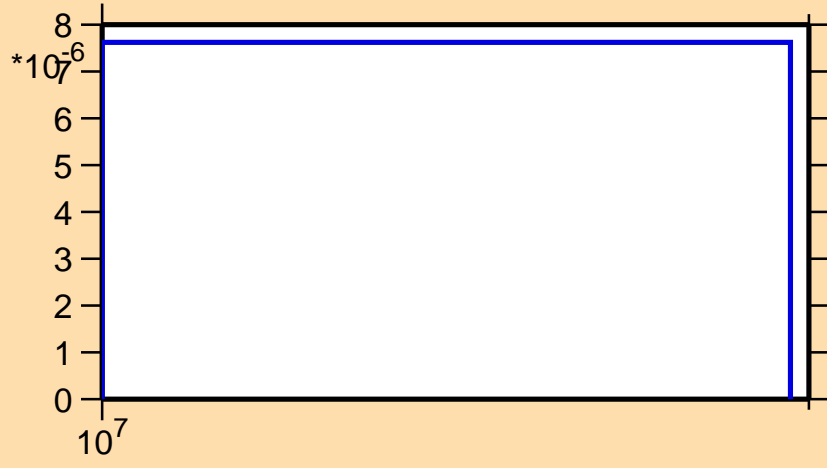
\sigma vs. E for ^{86}\text{Mo}(n,t)
