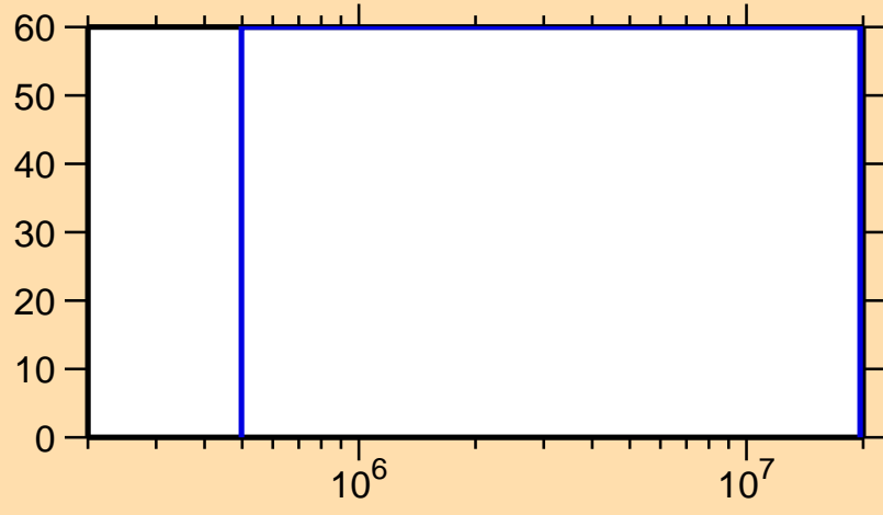
\Delta\sigma/\sigma vs. E for ^{86}\text{Mo}(n,\text{inel.})
