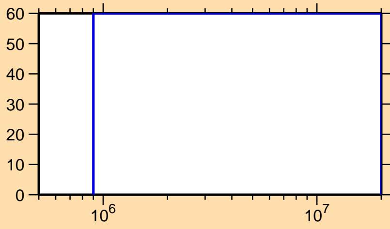
\Delta\sigma/\sigma vs. E for ^{86}\text{Mo}(n,n_1)
