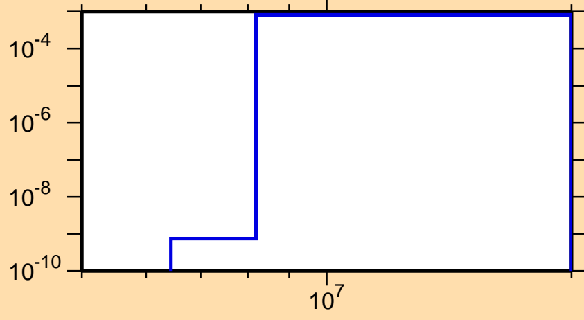
\sigma vs. E for ^{86}\text{Mo}(n,n\alpha)
