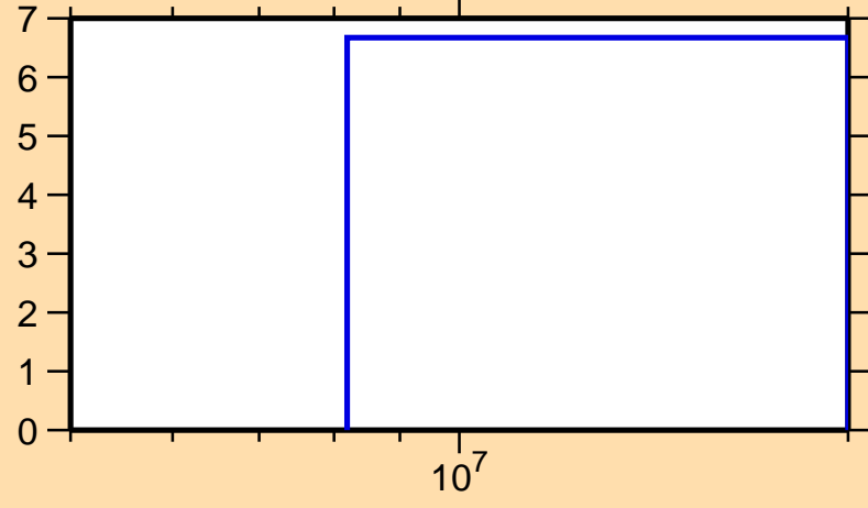
\Delta\sigma/\sigma vs. E for ^{86}\text{Mo}(n,\text{nonel.})
