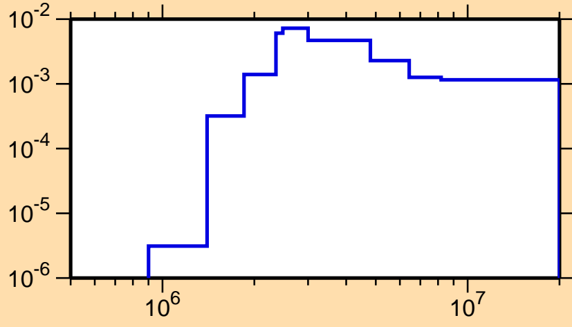
\sigma vs. E for ^{86}\text{Mo}(n,n\text{cont.})
