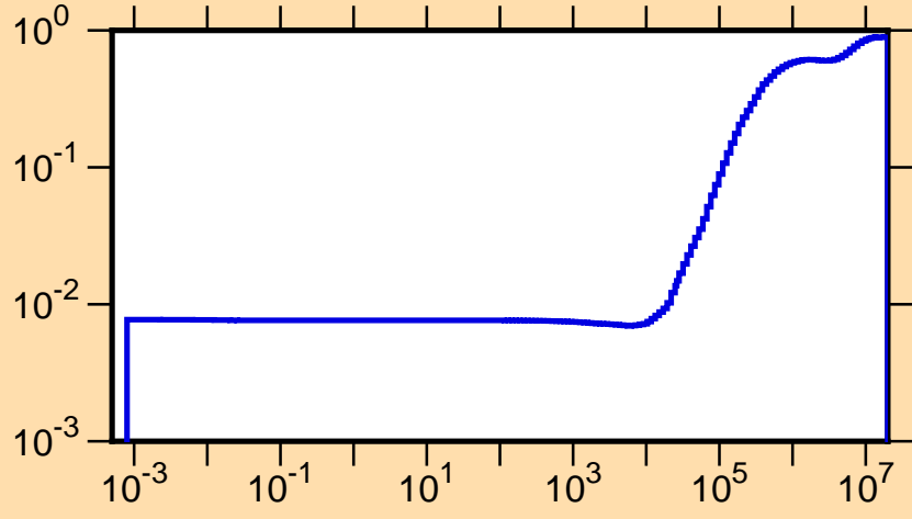
\mu vs. E for ^{87}\text{Mo}(\text{mt251})
