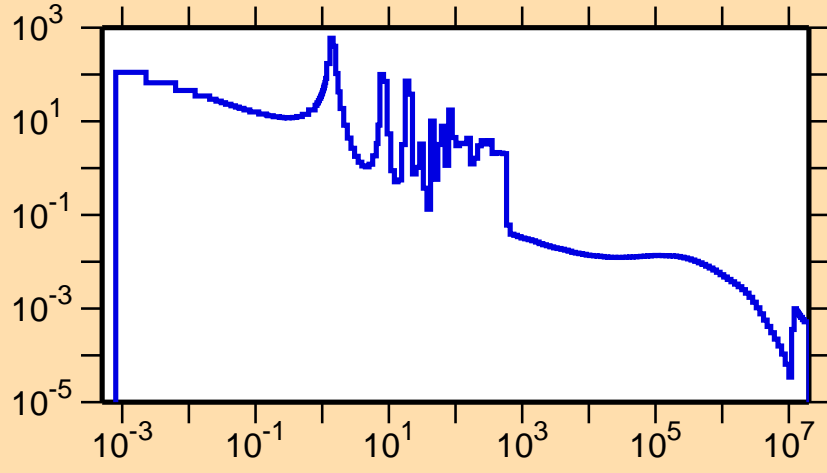
\sigma vs. E for ^{87}\text{Mo}(n,\gamma)
