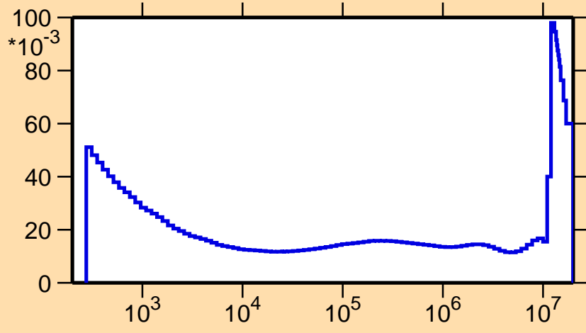
\sigma vs. E for ^{87}\text{Mo}(n,\alpha)
