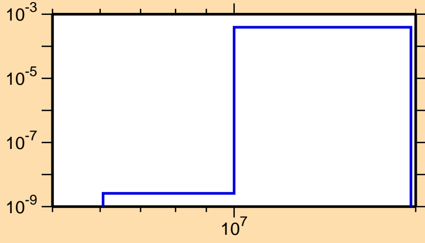
\sigma vs. E for ^{87}\text{Mo}(n,n\alpha)
