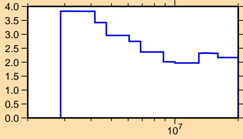
\Delta\sigma/\sigma vs. E for ^{88}\text{Mo}(n,n\text{onel.})
