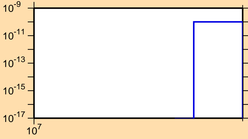
\sigma vs. E for ^{88}\text{Mo}(n,\text{nd})
