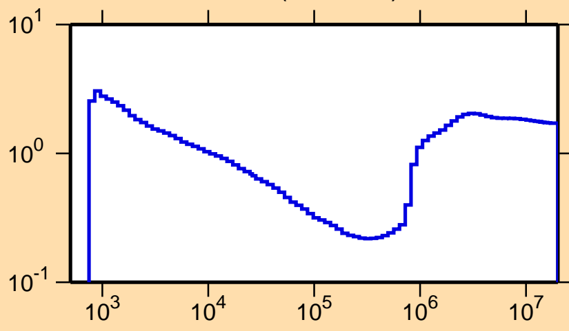
\sigma vs. E for ^{88}\text{Mo}(n,\text{nonel.})
