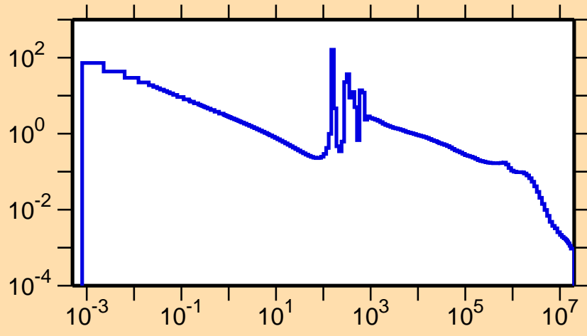
\sigma vs. E for ^{88}\text{Mo}(n,\gamma)
