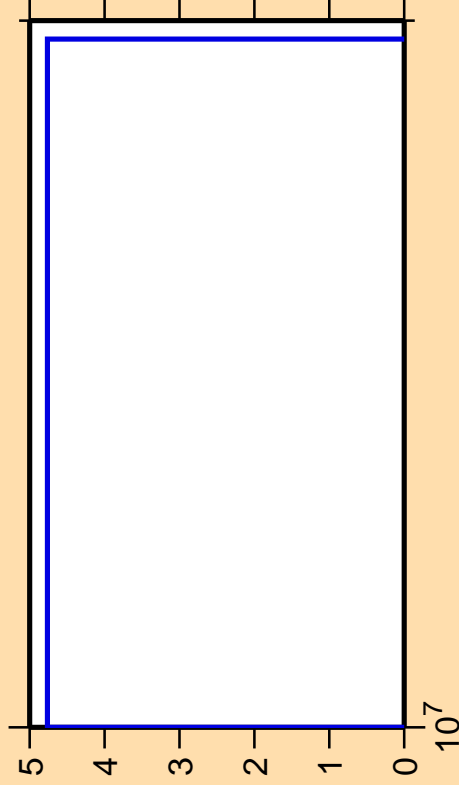
\Delta\sigma/\sigma vs. E for ^{88}\text{Mo}(\text{mt117})
