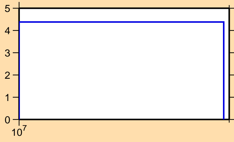
\Delta\sigma/\sigma vs. E for ^{88}\text{Mo}(n,\text{tot.})
