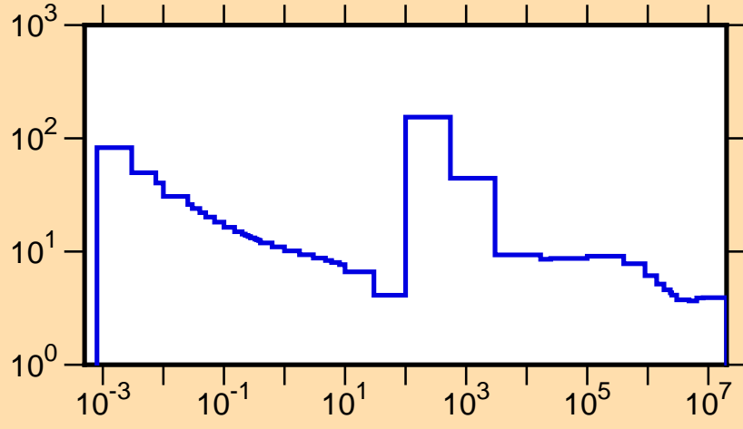
\sigma vs. E for ^{88}\text{Mo}(n,\text{tot.})
