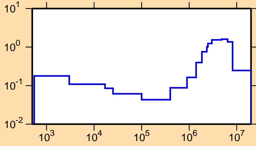
\sigma vs. E for ^{88}\text{Mo}(n,p)
