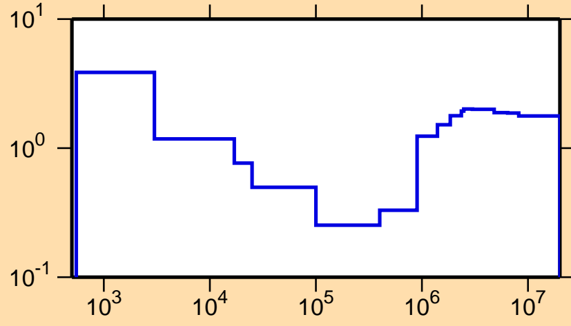
\sigma vs. E for ^{88}\text{Mo}(n,\text{nonel.})
