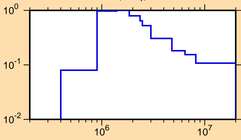
\sigma vs. E for ^{88}\text{Mo}(n,n_1)
