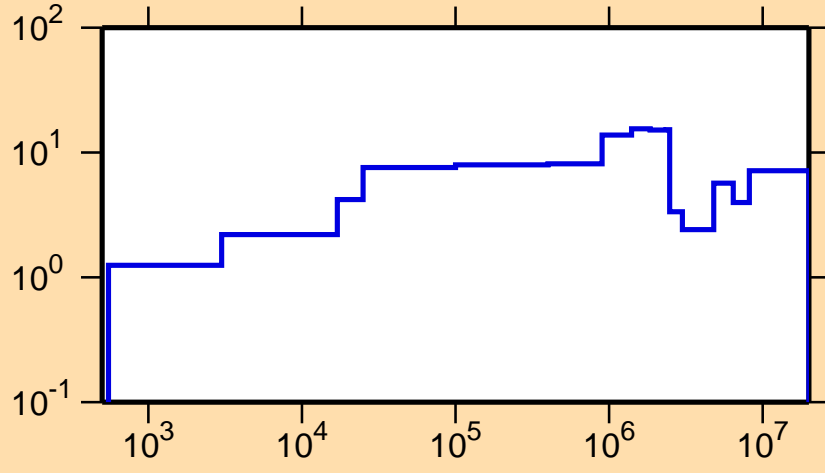
\Delta\sigma/\sigma vs. E for ^{88}\text{Mo}(n,el.)
