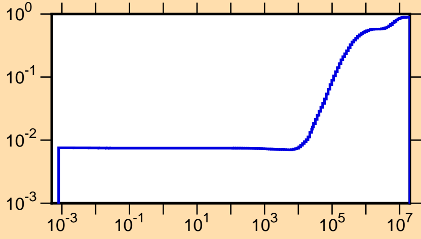
\mu vs. E for ^{89}\text{Mo}(\text{mt251})
