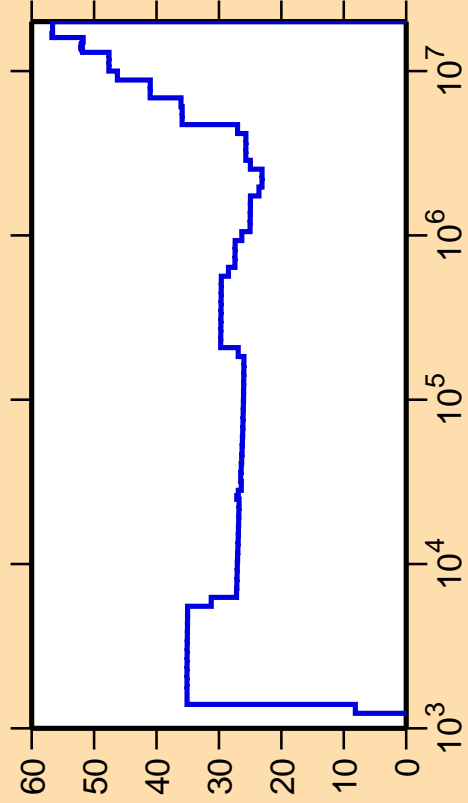
\Delta\sigma/\sigma vs. E for ^{89}\text{Mo}(n,\alpha)
