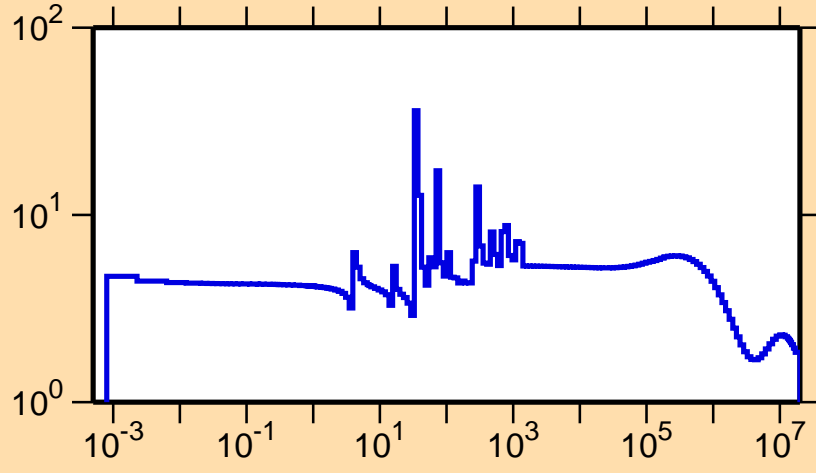
\sigma vs. E for ^{89}\text{Mo}(n,\text{el.})
