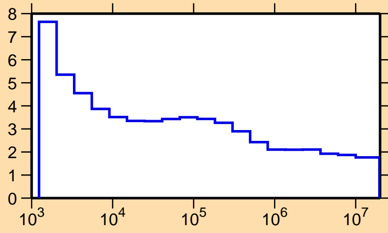
\sigma vs. E for ^{89}\text{Mo}(n,\text{nonel.})
