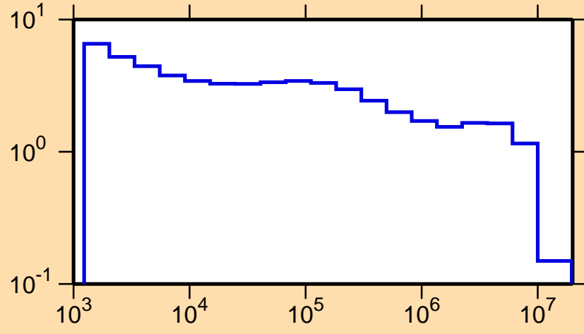
\sigma vs. E for ^{89}\text{Mo}(n,p)
