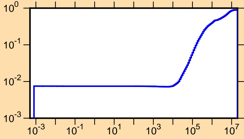
\mu vs. E for ^{90}\text{Mo}(\text{mt251})
