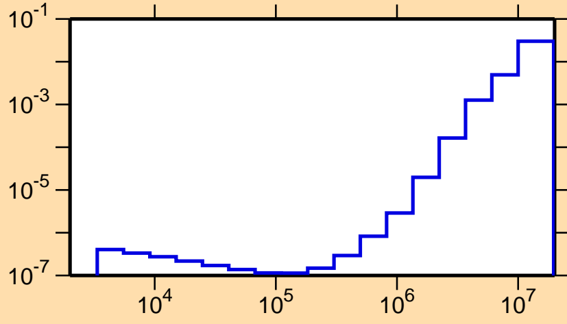
\sigma vs. E for ^{90}\text{Mo}(n,\alpha)
