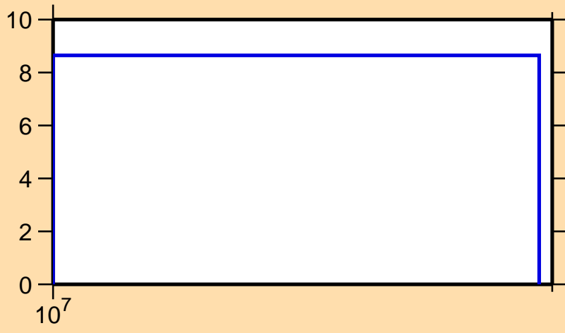
\Delta\sigma/\sigma vs. E for ^{90}\text{Mo}(n,\text{tot.})
