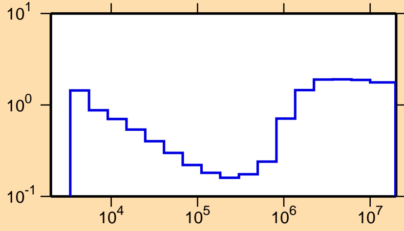
\sigma vs. E for ^{90}\text{Mo}(n,\text{nonel.})
