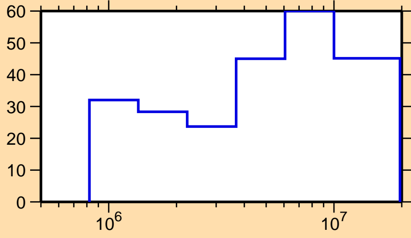
\Delta\sigma/\sigma vs. E for ^{90}\text{Mo}(n,n_1)
