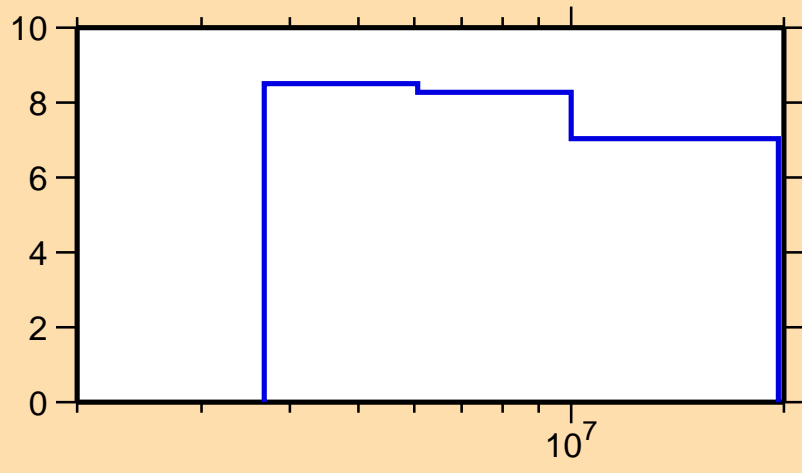
\Delta\sigma/\sigma vs. E for ^{90}\text{Mo}(n,n\text{inel.})
