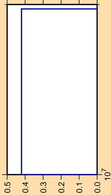
\Delta\sigma/\sigma vs. E for ^{90}\text{Mo} (mt 45)
