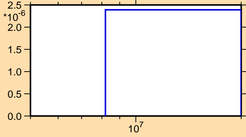
\sigma vs. E for ^{90}\text{Mo}(n,pd)
