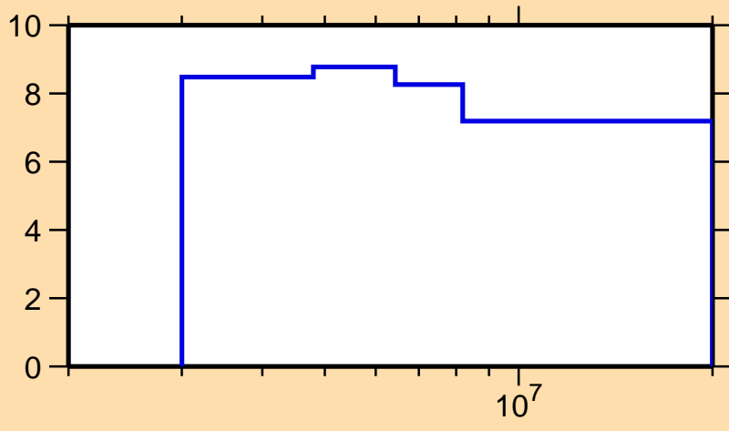
\Delta\sigma/\sigma vs. E for ^{90}\text{Mo}(n,n\text{onel.})
