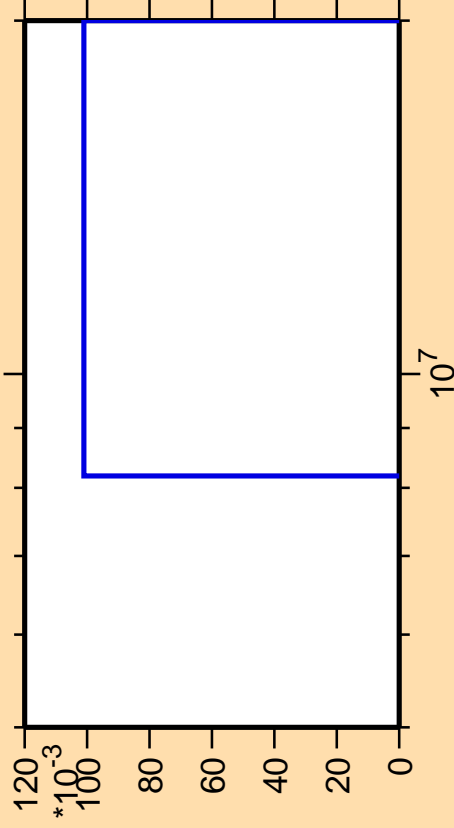
\Delta\sigma/\sigma vs. E for ^{90}\text{Mo}(\text{mt117})
