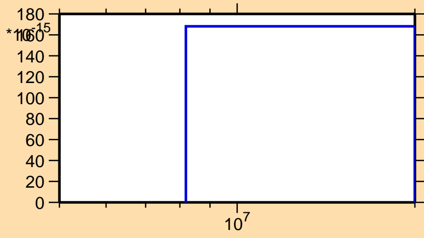
\sigma vs. E for ^{90}\text{Mo}(n,nd)
