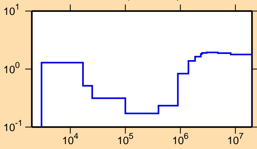
\sigma vs. E for ^{90}\text{Mo}(n,\text{nonel.})
