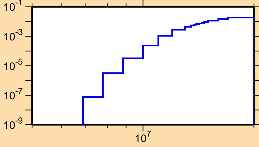
\sigma vs. E for ^{91}\text{Mo}(n,d)
