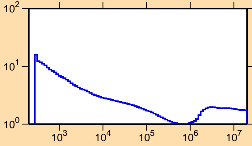
\sigma vs. E for ^{91}\text{Mo}(n,\text{nonel.})
