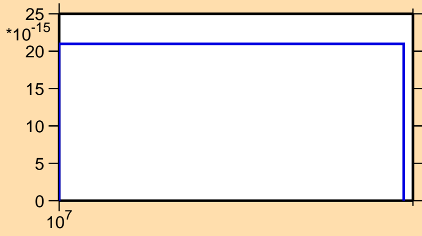
\sigma vs. E for ^{91}\text{Mo} (mt 34)
