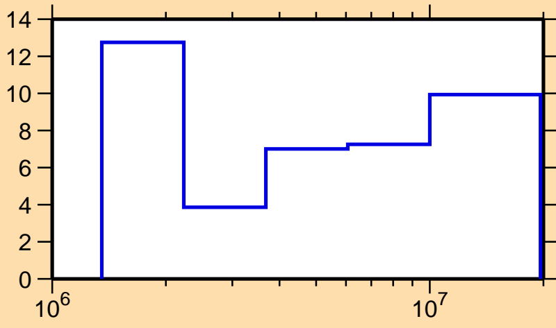
\Delta\sigma/\sigma vs. E for ^{92}\text{Mo}(n,\text{el.})
