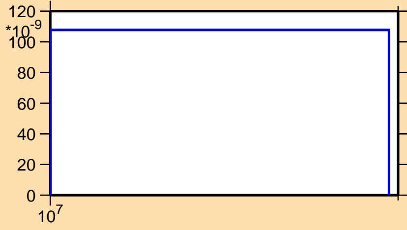
\sigma vs. E for ^{92}\text{Mo}(n,\text{pd})
