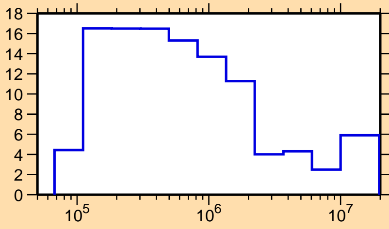
\Delta\sigma/\sigma vs. E for ^{92}\text{Mo}(n,\text{tot.})
