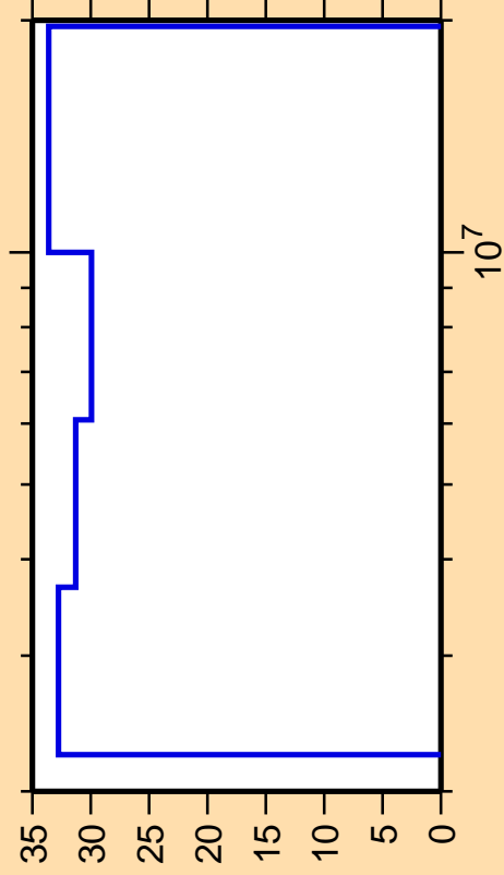
\Delta\sigma/\sigma vs. E for ^{92}\text{Mo}(n,n_4)
