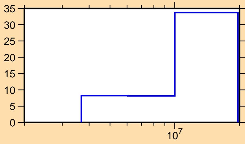
\Delta\sigma/\sigma vs. E for ^{92}\text{Mo}(n,n\text{cont.})
