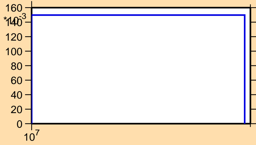
\sigma vs. E for ^{92}\text{Mo}(n,2n)
