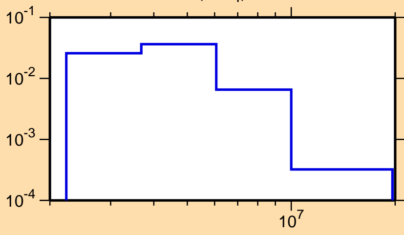
\sigma vs. E for ^{92}\text{Mo}(n,n_4)
