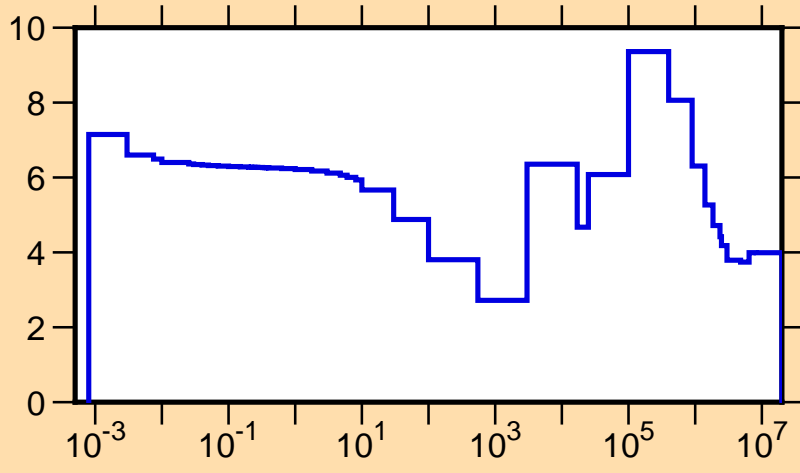
\sigma vs. E for ^{92}\text{Mo}(n,\text{tot.})
