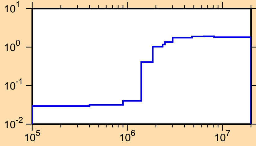
\sigma vs. E for ^{92}\text{Mo}(n,\text{nonel.})
