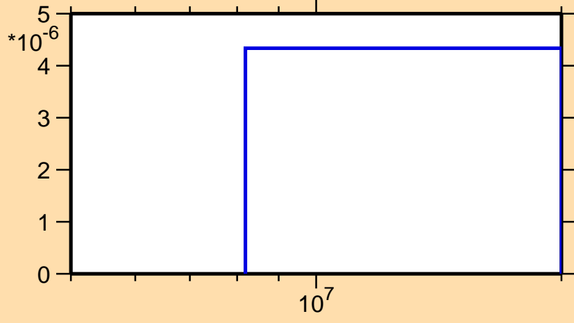
\sigma vs. E for ^{92}\text{Mo}(n,p\alpha)
