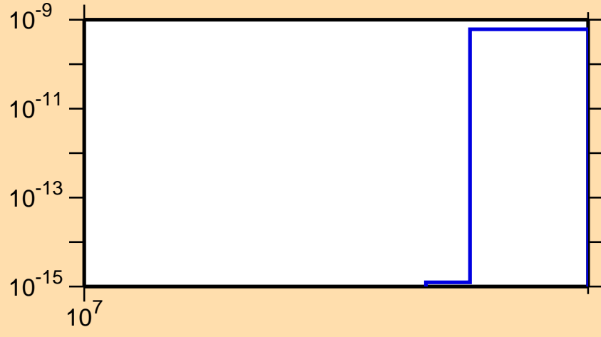
\sigma vs. E for ^{93}\text{Mo}(n,2n\alpha)
