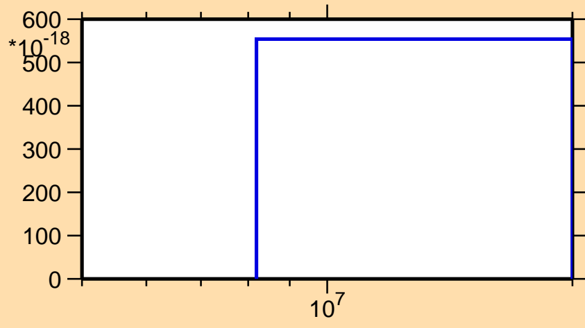
\sigma vs. E for ^{93}\text{Mo}(\text{mt117})
