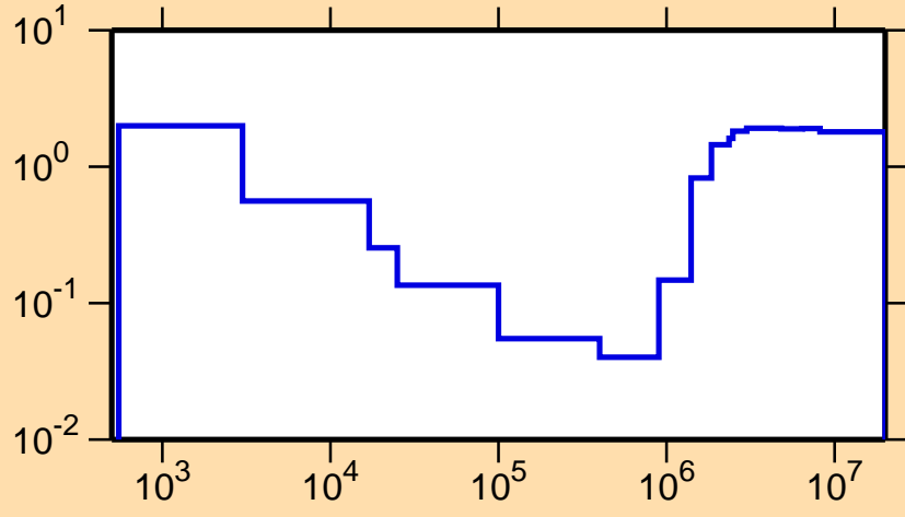
\sigma vs. E for ^{93}\text{Mo}(n,\text{nonel.})
