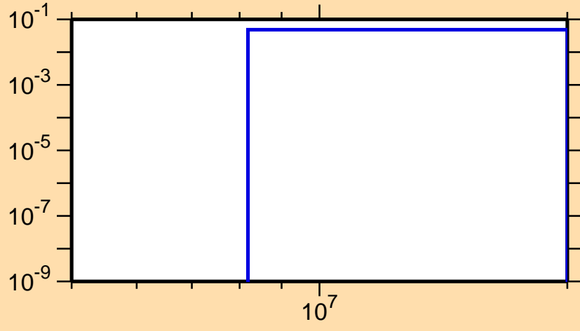
\sigma vs. E for ^{93}\text{Mo}(n,np)
