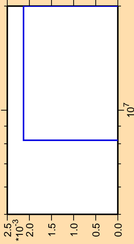
\Delta\sigma/\sigma vs. E for ^{93}\text{Mo}(\text{mt117})
