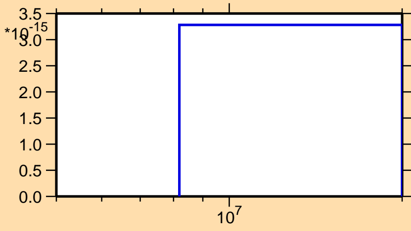
\sigma vs. E for ^{93}\text{Mo}(\text{mt } 45)
