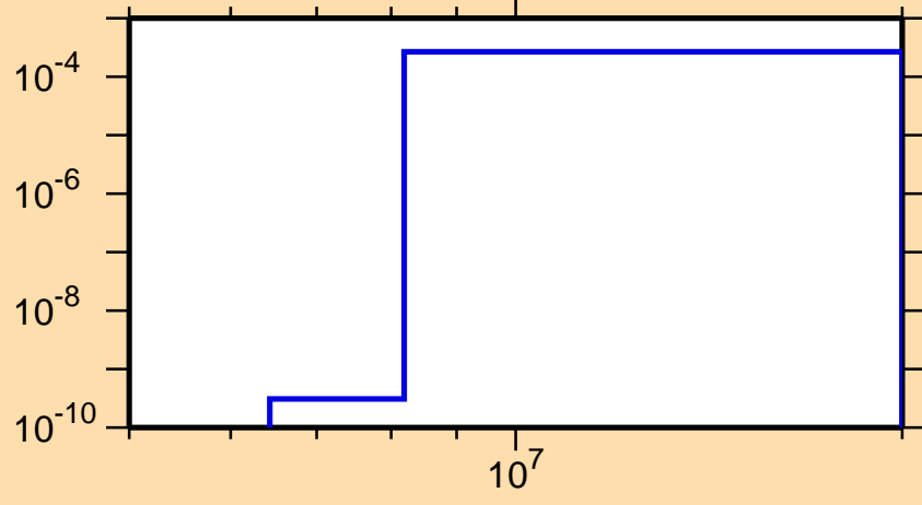
\sigma vs. E for ^{93}\text{Mo}(n,p\alpha)
