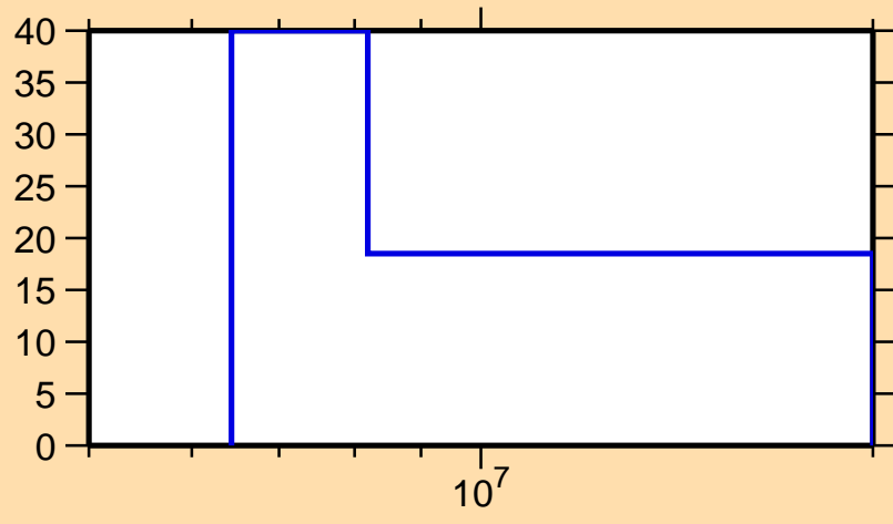
\Delta\sigma/\sigma vs. E for ^{93}\text{Mo}(n,2n)
