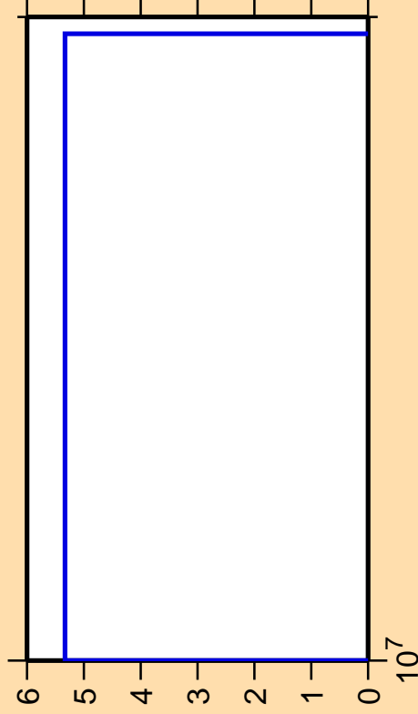
\Delta\sigma/\sigma vs. E for ^{93}\text{Mo}(n,nt)
