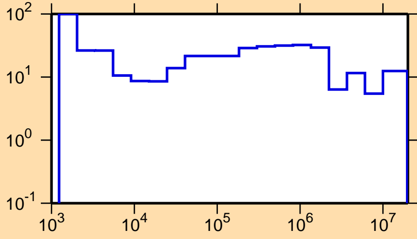
\Delta\sigma/\sigma vs. E for ^{93}\text{Mo}(n,el.)
