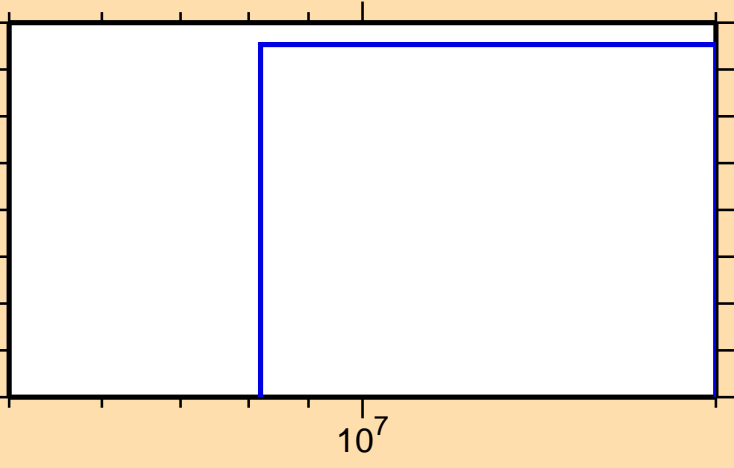
\sigma vs. E for ^{93}\text{Mo}(n,\text{He3})
