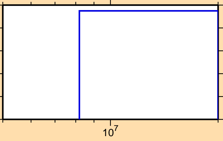
\sigma vs. E for ^{93}\text{Mo}(n,pd)
