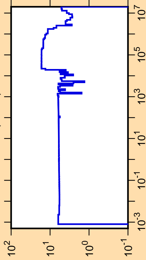
\Delta\sigma/\sigma vs. E for ^{94}\text{Mo}(n,\text{tot.})
