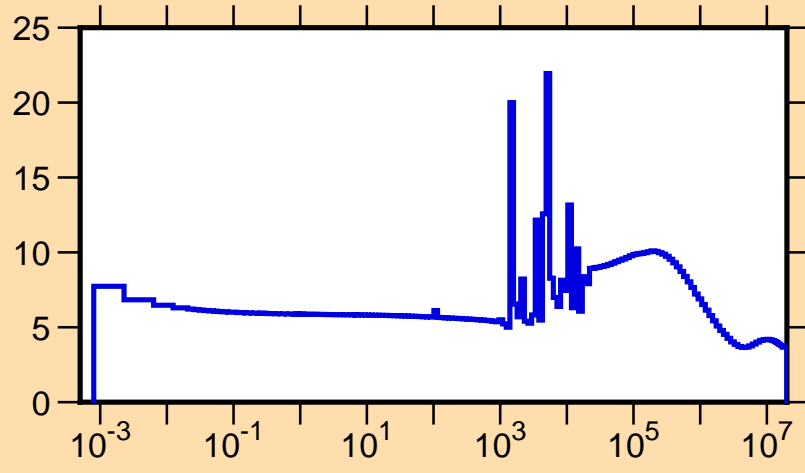
\sigma vs. E for ^{94}\text{Mo}(n,\text{tot.})
