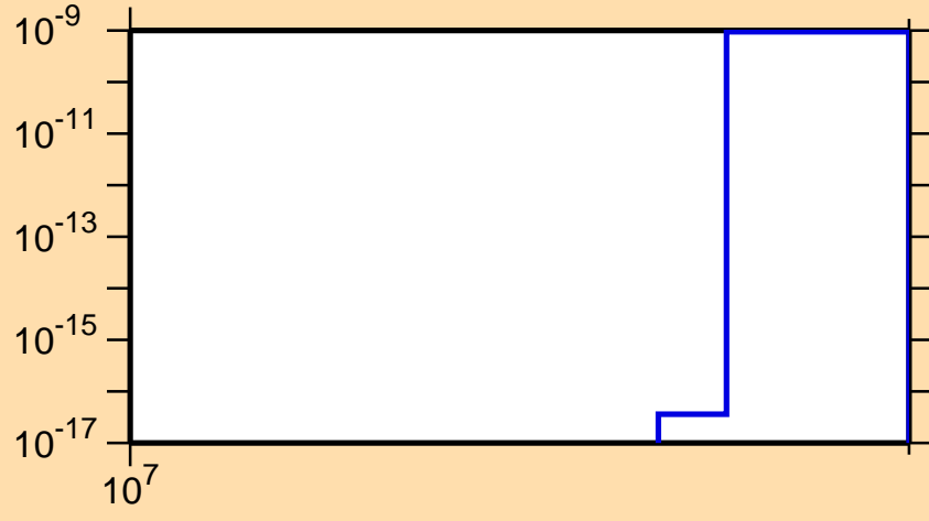
\sigma vs. E for ^{94}\text{Mo}(n,2n\alpha)
