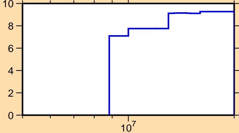
\Delta\sigma/\sigma vs. E for ^{94}\text{Mo}(n,\text{el.})
