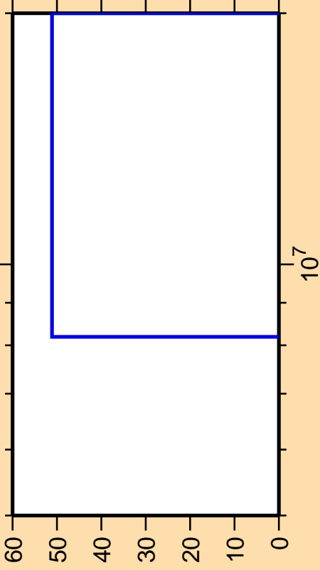
\Delta\sigma/\sigma vs. E for ^{94}\text{Mo}(n,3n)
