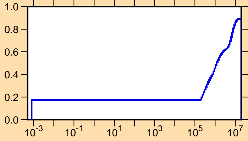
\mu vs. E for ^{95}\text{Mo}(\text{mt251})
