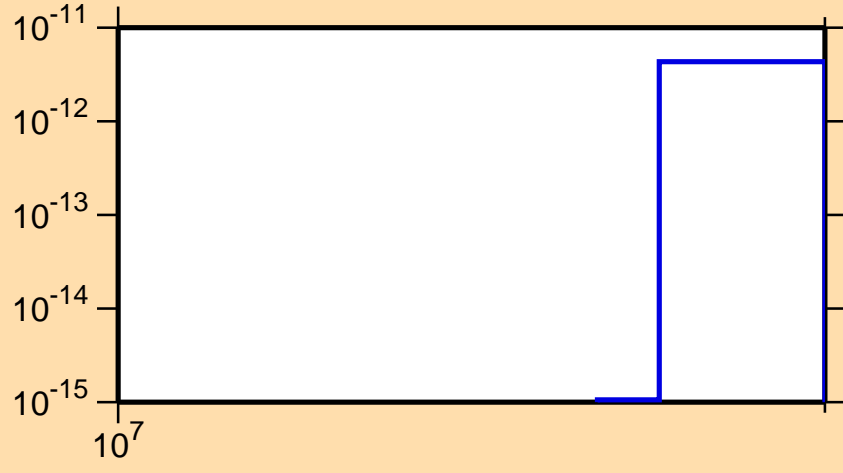
\sigma vs. E for ^{95}\text{Mo} (mt 45)
