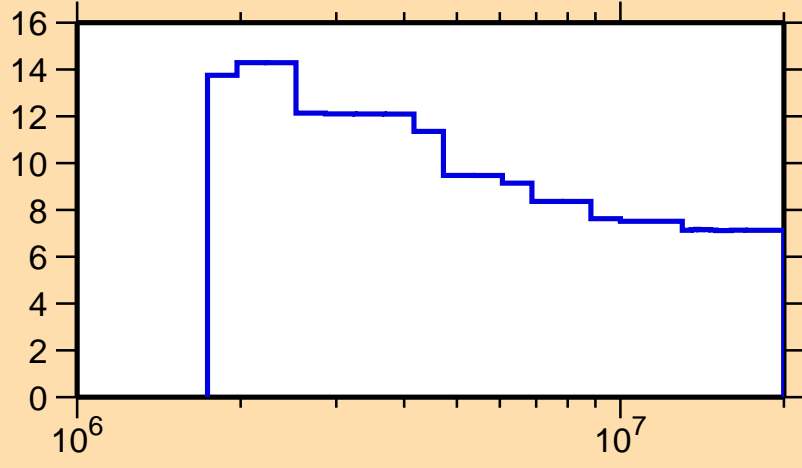
\Delta\sigma/\sigma vs. E for ^{95}\text{Mo}(n,n\text{onel.})
