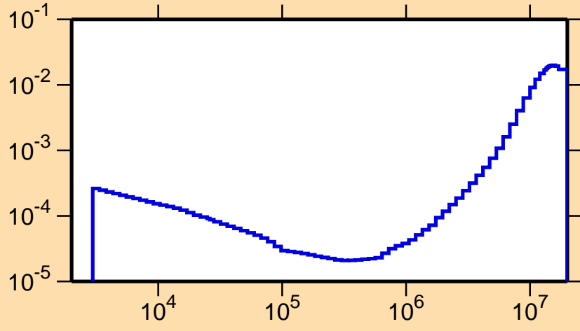
\sigma vs. E for ^{95}\text{Mo}(n,\alpha)
