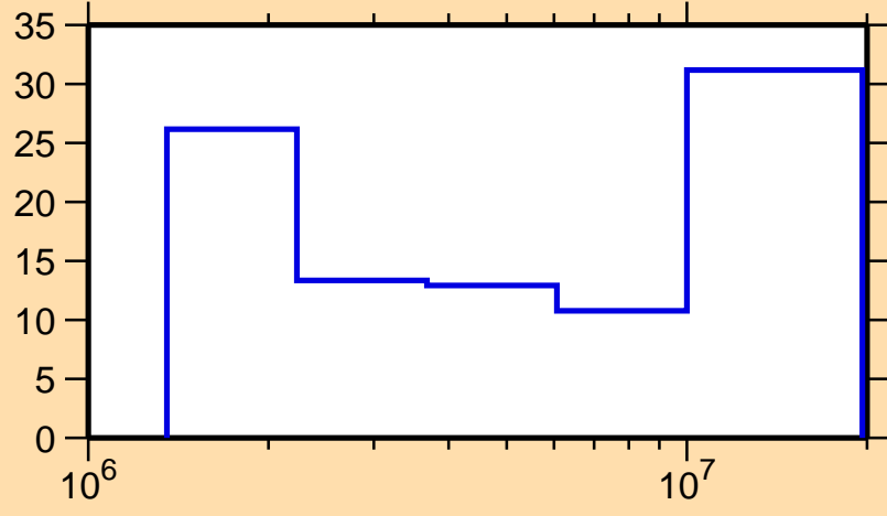
\Delta\sigma/\sigma vs. E for ^{95}\text{Mo}(n,n\text{cont.})
