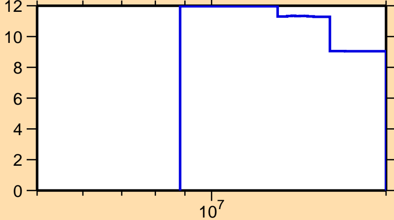
\Delta\sigma/\sigma vs. E for ^{96}\text{Mo}(n,2n)
