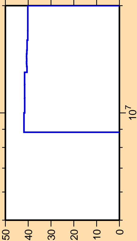
\Delta\sigma/\sigma vs. E for ^{96}\text{Mo}(n,n_1)
