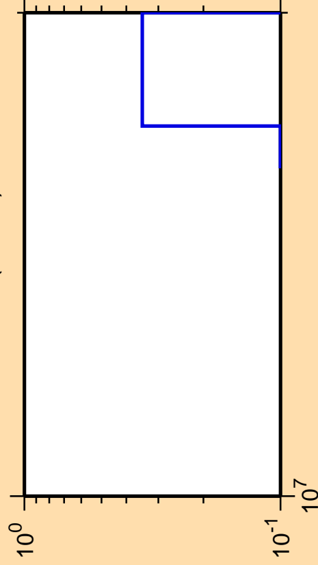
\Delta\sigma/\sigma vs. E for ^{96}\text{Mo} (mt 45)
