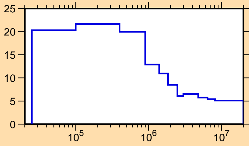
\Delta\sigma/\sigma vs. E for ^{96}\text{Mo}(n,\text{nonel.})
