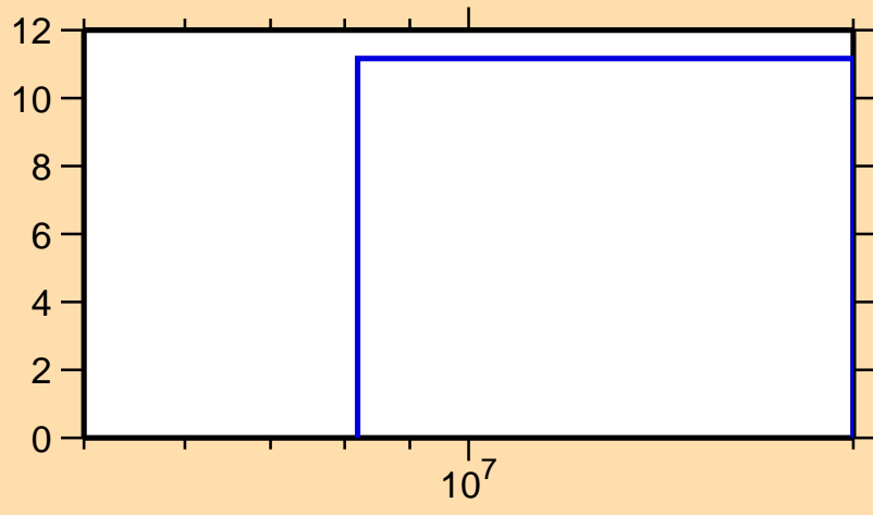
\Delta\sigma/\sigma vs. E for ^{96}\text{Mo}(n,2n)
