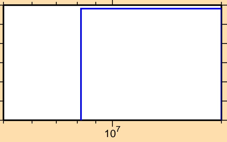
\sigma vs. E for ^{96}\text{Mo}(n,2n\alpha)
