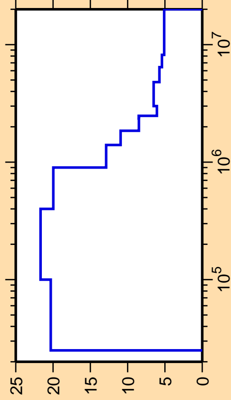
\Delta\sigma/\sigma vs. E for ^{96}\text{Mo}(n,\text{nonel.})
