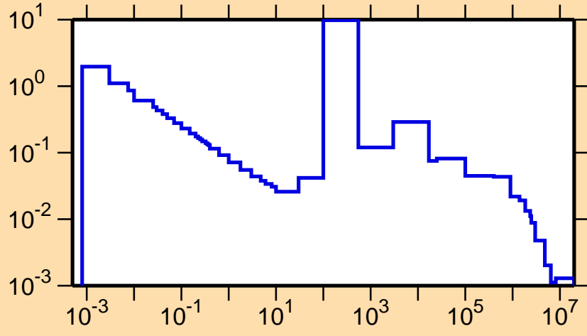
\sigma vs. E for ^{96}\text{Mo}(n,\gamma)
