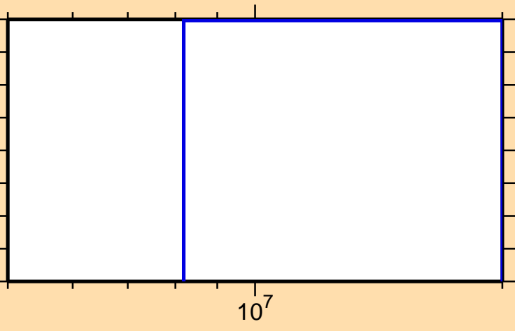
\sigma vs. E for ^{96}\text{Mo}(n,\text{He3})
