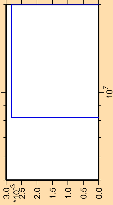
\Delta\sigma/\sigma vs. E for ^{96}\text{Mo}(\text{mt } 45)
