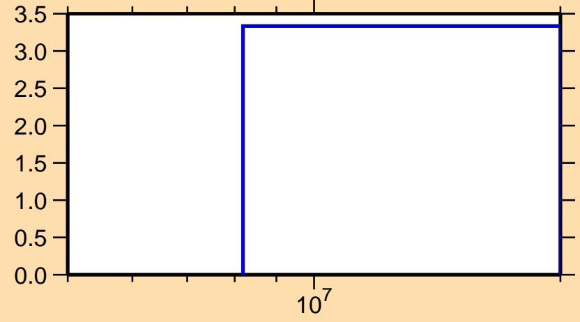
\Delta\sigma/\sigma vs. E for ^{96}\text{Mo}(n,\text{tot.})
