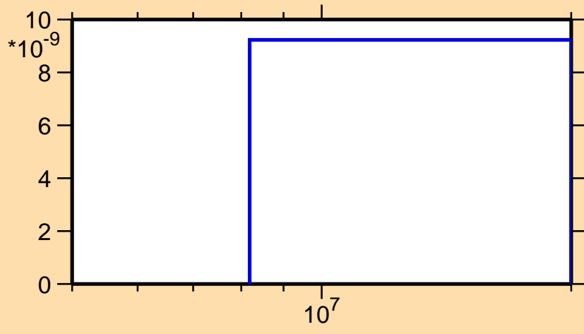
\sigma vs. E for ^{96}\text{Mo}(n,\text{nd})
