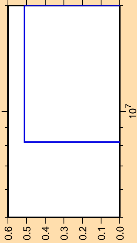
\Delta\sigma/\sigma vs. E for ^{96}\text{Mo}(\text{mt117})
