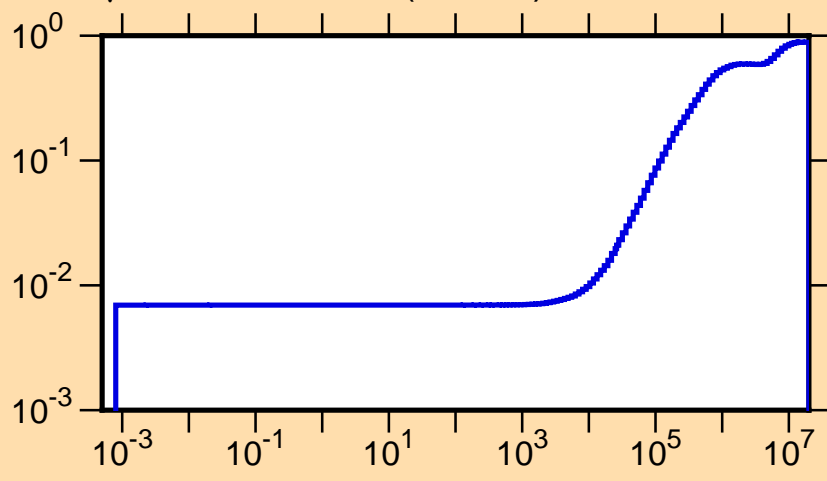
\mu vs. E for ^{97}\text{Mo}(\text{mt251})
