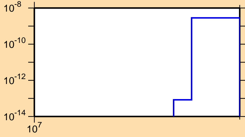
\sigma vs. E for ^{97}\text{Mo}(n,nt)
