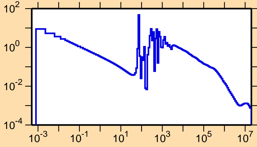
\sigma vs. E for ^{97}\text{Mo}(n,\gamma)
