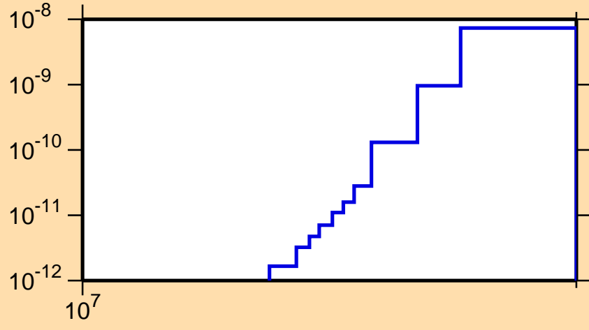
\sigma vs. E for ^{97}\text{Mo}(n,p\alpha)
