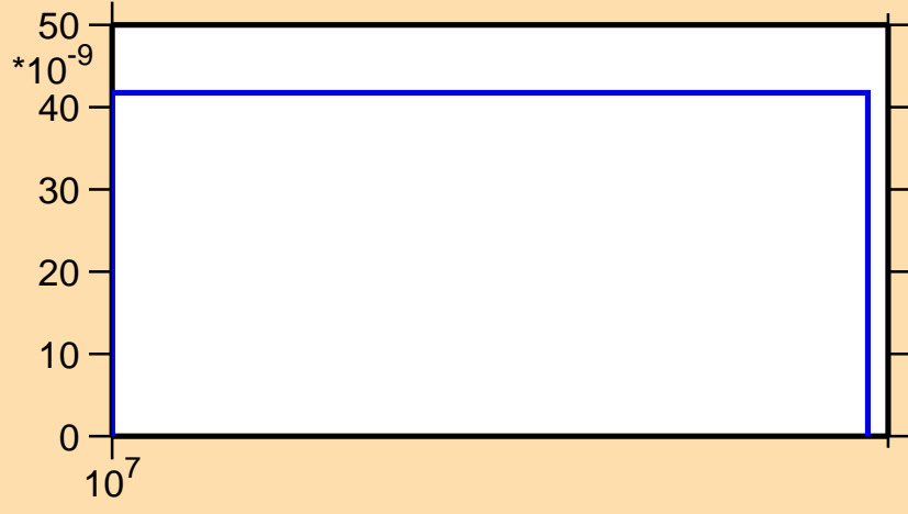
\sigma vs. E for ^{97}\text{Mo}(n,\text{nd})
