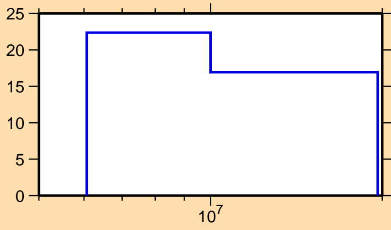
\Delta\sigma/\sigma vs. E for ^{97}\text{Mo}(n,2n)
