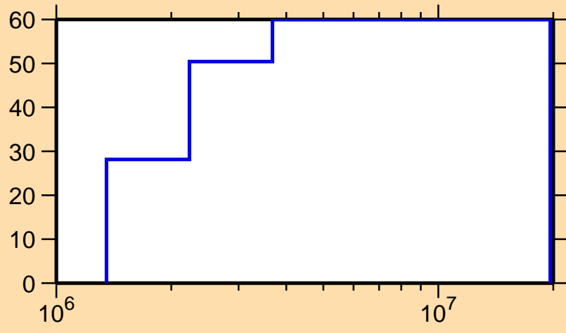
\Delta\sigma/\sigma vs. E for ^{97}\text{Mo}(n,\gamma)
