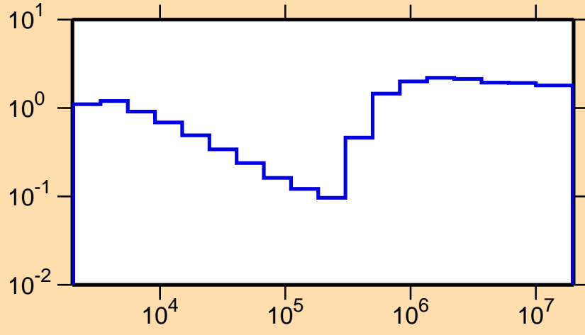
\sigma vs. E for ^{97}\text{Mo}(n,\text{nonel.})
