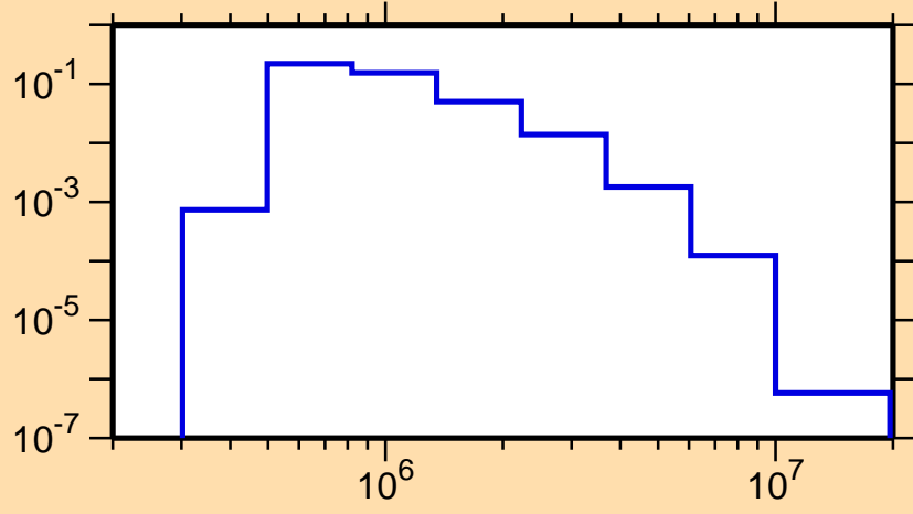
\sigma vs. E for ^{97}\text{Mo}(n,n_4)
