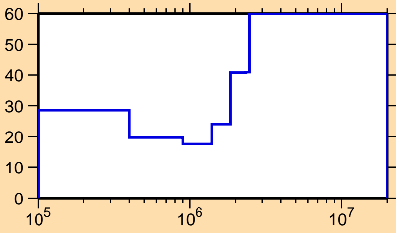
\Delta\sigma/\sigma vs. E for ^{97}\text{Mo}(n,n_1)
