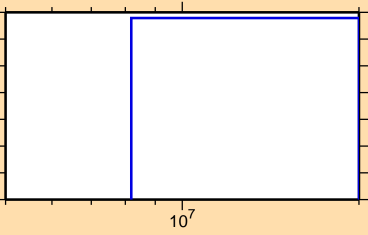
\sigma vs. E for ^{97}\text{Mo}(n,2n\alpha)
