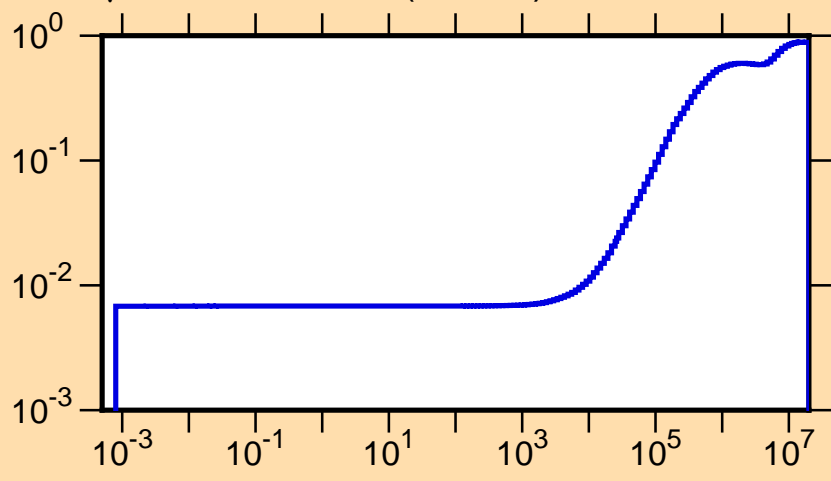
\mu vs. E for ^{99}\text{Mo}(\text{mt251})
