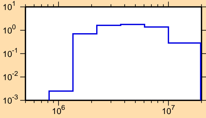
\sigma vs. E for ^{99}\text{Mo}(n,n\text{cont.})
