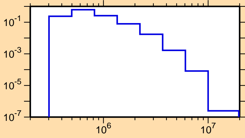
\sigma vs. E for ^{99}\text{Mo}(n,n_3)
