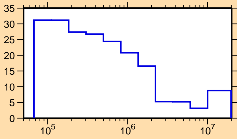
\Delta\sigma/\sigma vs. E for ^{99}\text{Mo}(n,\text{tot.})
