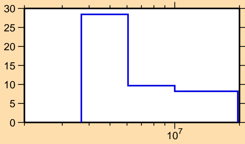
\Delta\sigma/\sigma vs. E for ^{99}\text{Mo}(n,2n)
