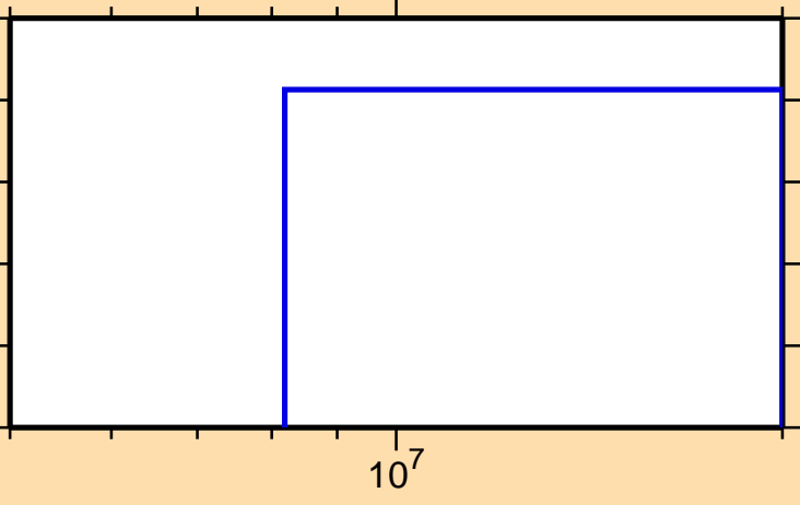
\sigma vs. E for ^{99}\text{Mo}(n,\text{nd})
