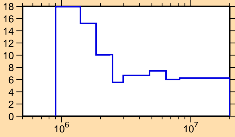
\Delta\sigma/\sigma vs. E for ^{99}\text{Mo}(n,n\text{onel.})
