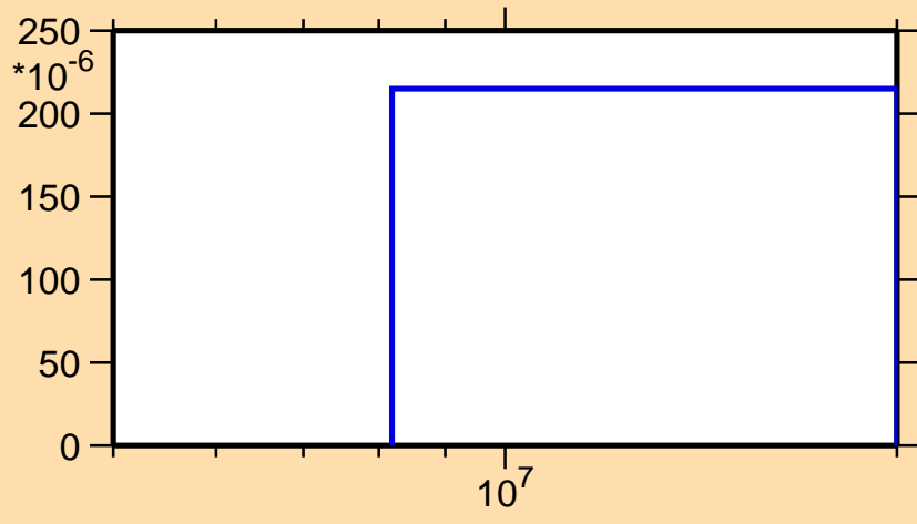
\sigma vs. E for ^{99}\text{Mo}(n,t)
