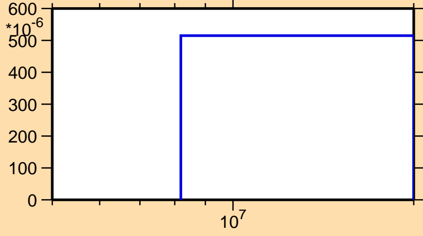
\sigma vs. E for ^{99}\text{Mo}(n,d)
