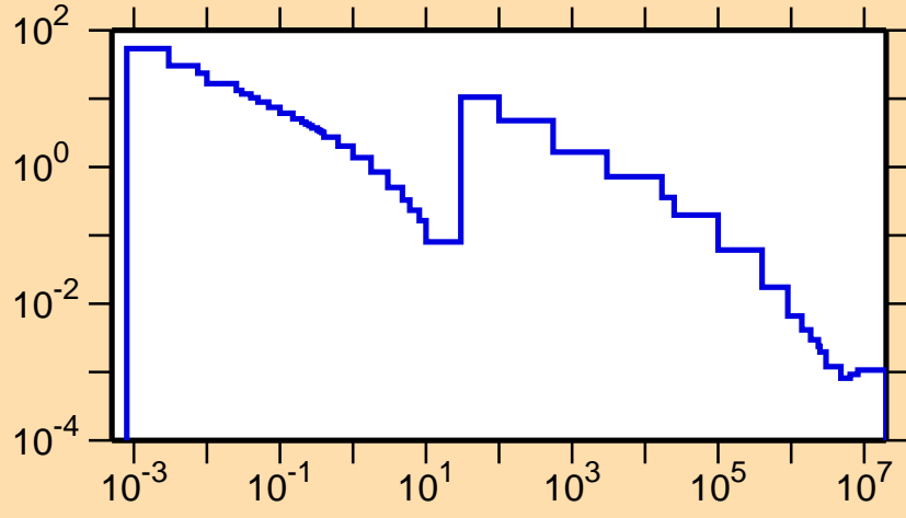
\sigma vs. E for ^{99}\text{Mo}(n,\gamma)
