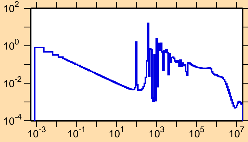
\sigma vs. E for ^{100}\text{Mo}(n,\gamma)
