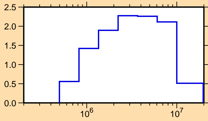
\sigma vs. E for ^{100}\text{Mo}(n,\text{inel.})
