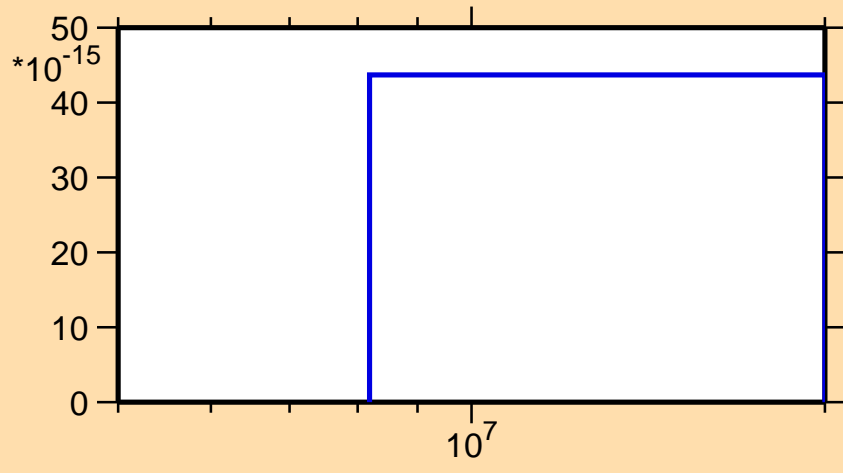
\sigma vs. E for ^{100}\text{Mo}(n,2np)
