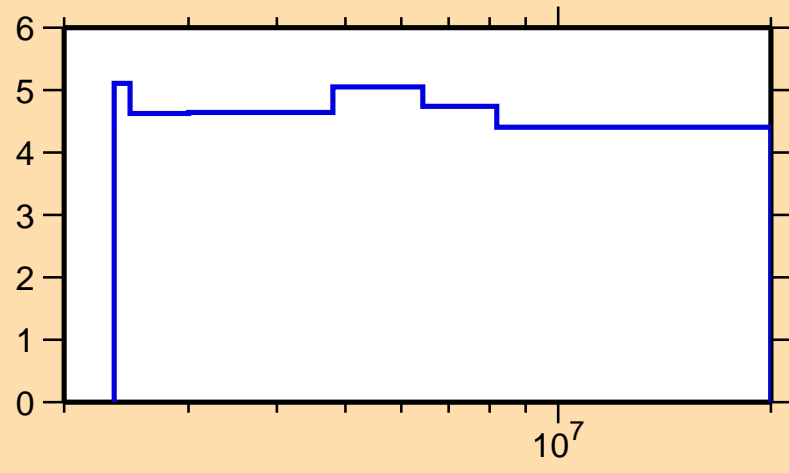
\Delta\sigma/\sigma vs. E for ^{100}\text{Mo}(n,n\text{onel.})
