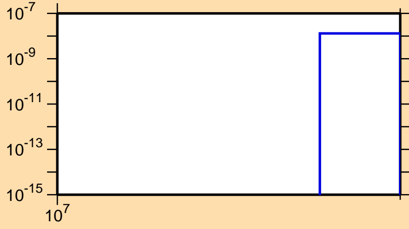
\sigma vs. E for ^{101}\text{Mo}(n,2np)
