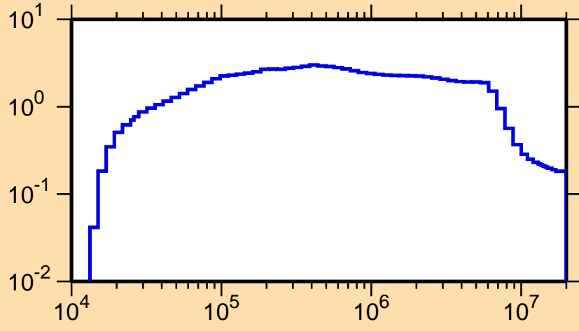
\sigma vs. E for ^{101}\text{Mo}(n,\text{inel.})
