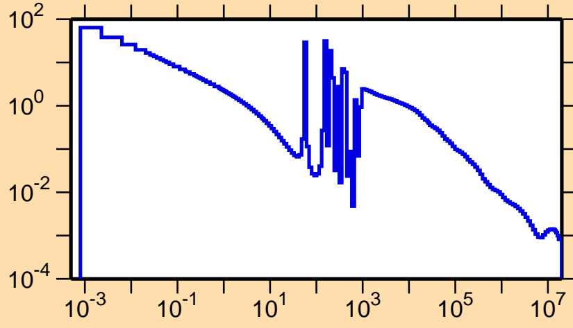
\sigma vs. E for ^{101}\text{Mo}(n,\gamma)
