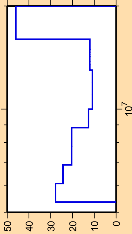
\Delta\sigma/\sigma vs. E for ^{101}\text{Mo}(n,2n)
