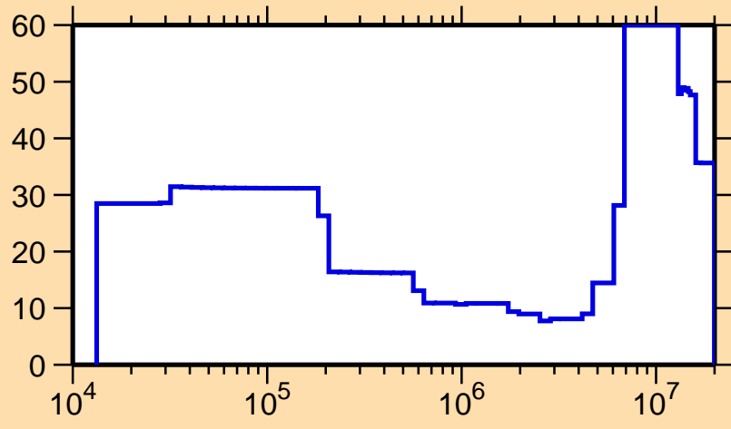
\Delta\sigma/\sigma vs. E for ^{101}\text{Mo}(n,\text{inel.})
