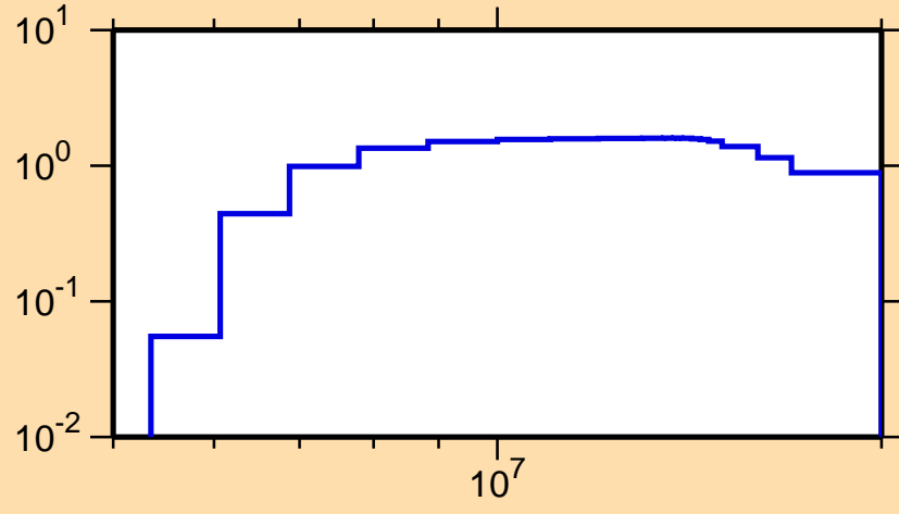
\sigma vs. E for ^{101}\text{Mo}(n,2n)
