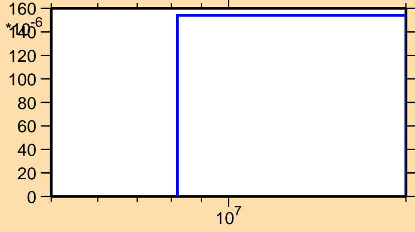
\sigma vs. E for ^{101}\text{Mo}(n,d)
